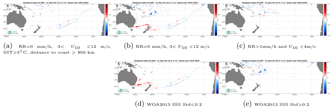
Figure 12: Temporal mean gridded over spatial boxes of size 1^\circ \times 1^\circ of \Delta SSS (SMAP SSS L3 v4 - Monthly (RSS) - TSG (LEGOS-DM)) for 5 different subdatasets corresponding to: RR=0 mm/h, 3 < U_{10} < 12 m/s, SST > 5^\circ\text{C} , distance to coast > 800 km (a), RR=0 mm/h, 3 < U_{10} < 12 m/s (b), RR > 1 mm/h and U_{10} < 4 m/s (c), WOA2013 SSS Std < 0.2 (d), WOA2013 SSS Std > 0.2 (e).
