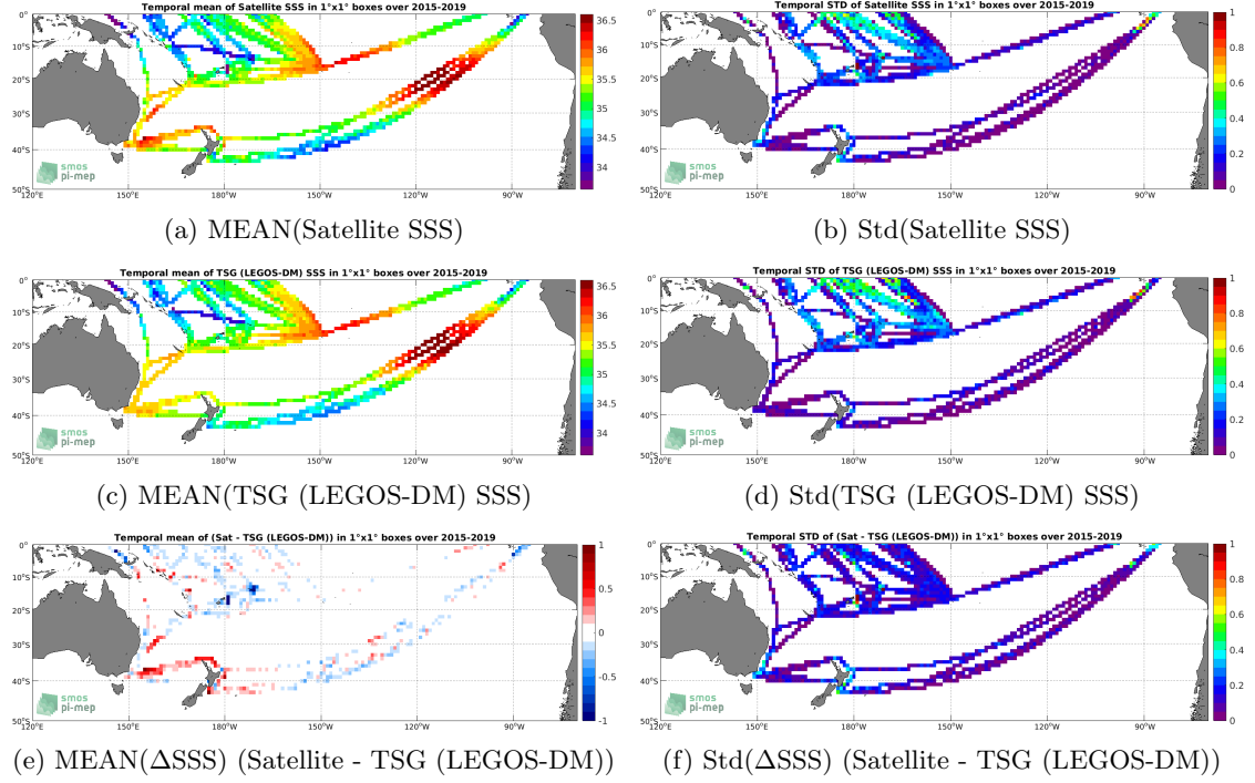
Figure 6: Temporal mean (left) and Std (right) of SSS from SMAP SSS L3 v4 - Monthly (RSS) (top), TSG (LEGOS-DM) (middle), and of \Delta SSS (Satellite - TSG (LEGOS-DM)). Only match-up pairs are used to generate these maps.
