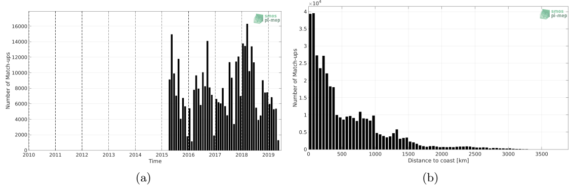
Figure 1: Number of match-ups between TSG (LEGOS-DM) and SMAP SSS L3 v4 - Monthly (RSS) SSS as a function of time (a) and as function of the distance to coast (b) over the South Pacific Ocean Pi-MEP region and for the full satellite product period.
