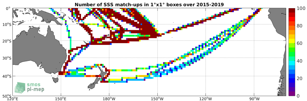
Figure 4: Number of SSS match-ups between TSG (LEGOS-DM) SSS and the SMAP SSS L3 v4 - Monthly (RSS) SSS product for the South Pacific Ocean Pi-MEP region over 1°x1° boxes and for the full satellite product period.
