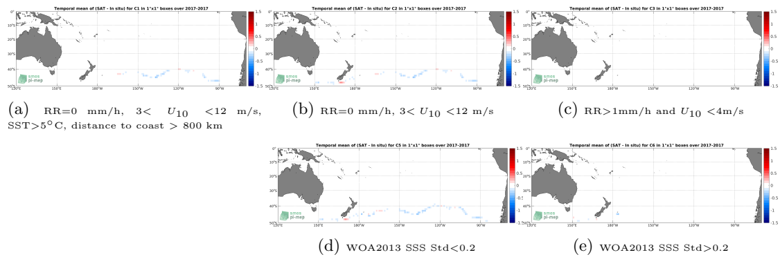
Figure 12: Temporal mean gridded over spatial boxes of size 1^\circ \times 1^\circ of \Delta\text{SSS} (SMAP SSS L3 v4 - Monthly (RSS) - TSG (GOSUD-Sailing-ship)) for 5 different subdatasets corresponding to:RR=0 mm/h, 3 < U_{10} < 12 m/s, SST > 5°C, distance to coast > 800 km (a), RR=0 mm/h, 3 < U_{10} < 12 m/s (b), RR > 1mm/h and U_{10} < 4 m/s (c), WOA2013 SSS Std < 0.2 (d), WOA2013 SSS Std > 0.2 (e).
