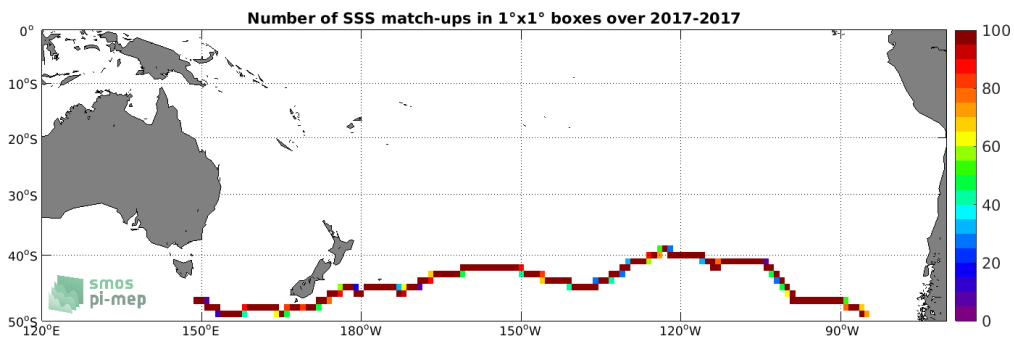
Figure 4: Number of SSS match-ups between TSG (GOSUD-Sailing-ship) SSS and the SMAP SSS L3 v4 - Monthly (RSS) SSS product for the South Pacific Ocean Pi-MEP region over 1^\circ \times 1^\circ boxes and for the full satellite product period.
