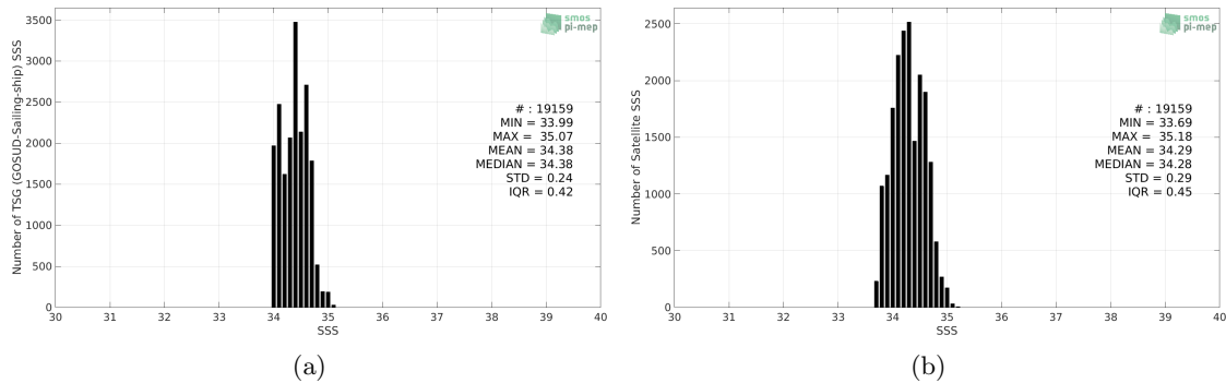
Figure 2: Histograms of SSS from TSG (GOSUD-Sailing-ship) (a) and SMAP SSS L3 v4 - Monthly (RSS) (b) considering all match-up pairs per bins of 0.1 over the South Pacific Ocean Pi-MEP region and for the full satellite product period.
