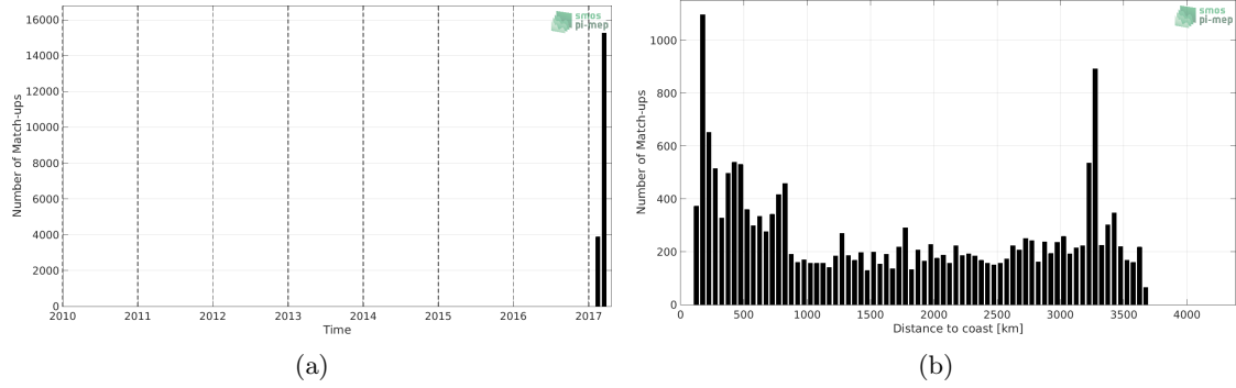
Figure 1: Number of match-ups between TSG (GOSUD-Sailing-ship) and SMAP SSS L3 v4 - Monthly (RSS) SSS as a function of time (a) and as function of the distance to coast (b) over the South Pacific Ocean Pi-MEP region and for the full satellite product period.
