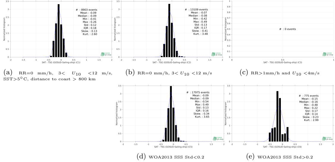
Figure 13: Normalized histogram of \Delta SSS (SMAP SSS L3 v4 - Monthly (RSS) - TSG (GOSUD-Sailing-ship)) for 5 different subdatasets corresponding to: RR=0 mm/h, 3 < U_{10} < 12 m/s, SST > 5°C, distance to coast > 800 km (a), RR=0 mm/h, 3 < U_{10} < 12 m/s (b), RR > 1mm/h and U_{10} < 4 m/s (c), WOA2013 SSS Std < 0.2 (d), WOA2013 SSS Std > 0.2 (e).
