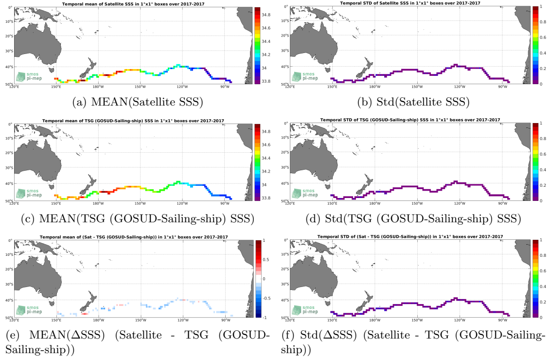
Figure 6: Temporal mean (left) and Std (right) of SSS from SMAP SSS L3 v4 - Monthly (RSS) (top), TSG (GOSUD-Sailing-ship) (middle), and of \Delta SSS (Satellite - TSG (GOSUD-Sailing-ship)). Only match-up pairs are used to generate these maps.
