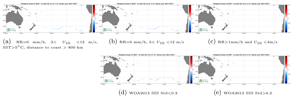
Figure 12: Temporal mean gridded over spatial boxes of size 1^\circ \times 1^\circ of \Delta SSS (SMAP-L3-RSS-V4-MONTHLY - TSG-GOSUD-Sailing-ship) for 5 different subdatasets corresponding to:RR=0 mm/h, 3 < U_{10} < 12 m/s, SST>5°C, distance to coast > 800 km (a), RR=0 mm/h, 3 < U_{10} < 12 m/s (b), RR>1mm/h and U_{10} < 4 m/s (c), WOA2013 SSS Std<0.2 (d), WOA2013 SSS Std>0.2 (e).
