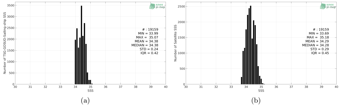
Figure 2: Histograms of SSS from TSG-GOSUD-Sailing-ship (a) and SMAP-L3-RSS-V4-MONTHLY (b) considering all match-up pairs per bins of 0.1 over the South Pacific Ocean Pi-MEP region and for the full satellite product period.
