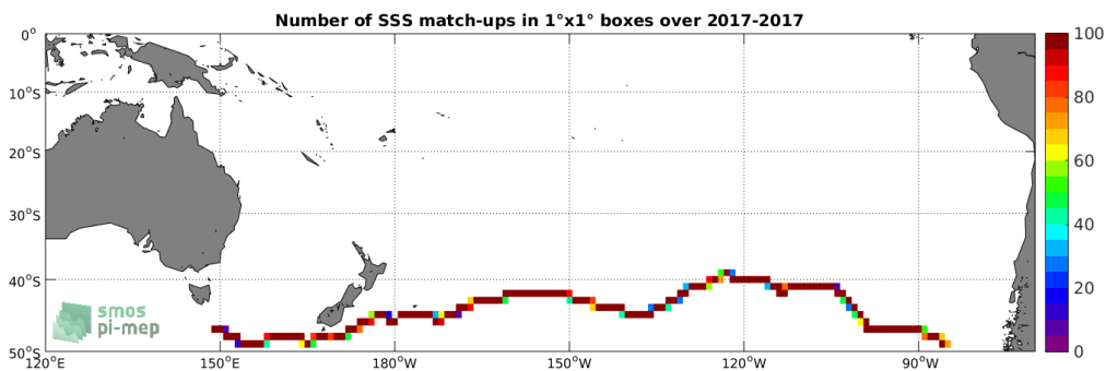
Figure 4: Number of SSS match-ups between TSG-GOSUD-Sailing-ship SSS and the SMAP-L3-RSS-V4-MONTHLY SSS product for the South Pacific Ocean Pi-MEP region over 1°x1° boxes and for the full satellite product period.
