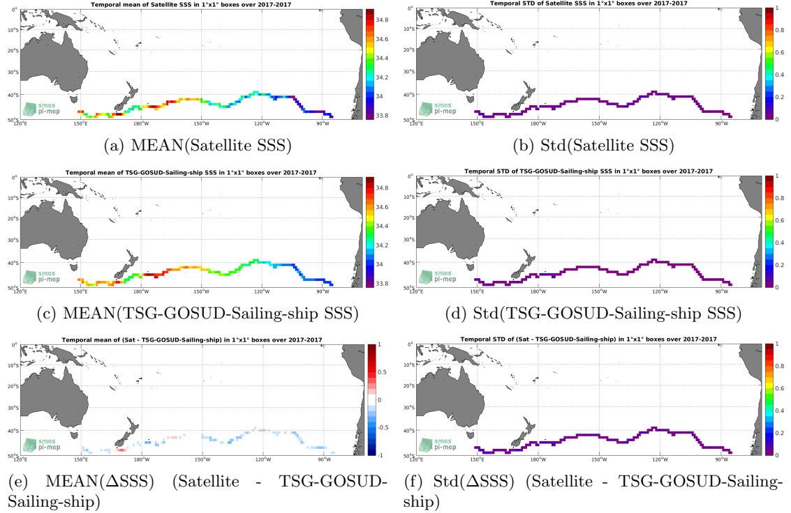
Figure 6: Temporal mean (left) and Std (right) of SSS from SMAP-L3-RSS-V4-MONTHLY (top), TSG-GOSUD-Sailing-ship (middle), and of \Delta SSS (Satellite - TSG-GOSUD-Sailing-ship). Only match-up pairs are used to generate these maps.
