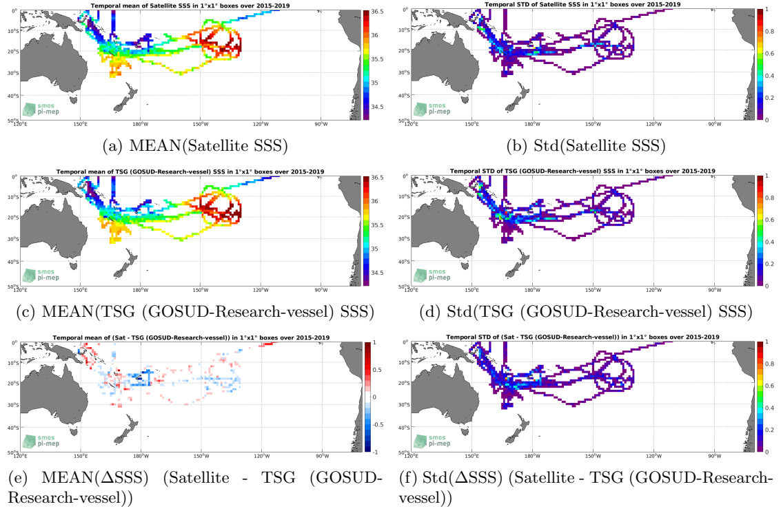
Figure 6: Temporal mean (left) and Std (right) of SSS from SMAP SSS L3 v4 - Monthly (RSS) (top), TSG (GOSUD-Research-vessel) (middle), and of \Delta SSS (Satellite - TSG (GOSUD-Research-vessel)). Only match-up pairs are used to generate these maps.
