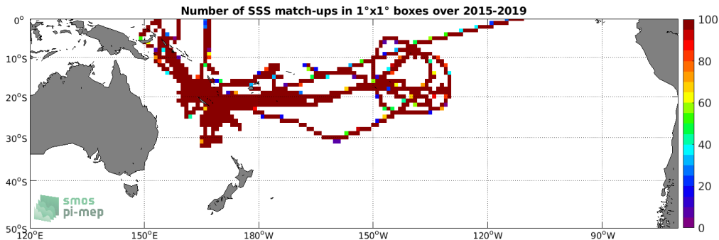
Figure 4: Number of SSS match-ups between TSG (GOSUD-Research-vessel) SSS and the SMAP SSS L3 v4 - Monthly (RSS) SSS product for the South Pacific Ocean Pi-MEP region over 1^\circ \times 1^\circ boxes and for the full satellite product period.
