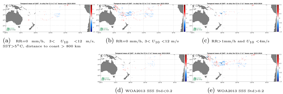
Figure 12: Temporal mean gridded over spatial boxes of size 1^\circ \times 1^\circ of \Delta SSS (SMAP SSS L3 v4 - Monthly (RSS) - TSG (GOSUD-Research-vessel)) for 5 different subdatasets corresponding to:RR=0 mm/h, 3 < U_{10} < 12 m/s, SST>5°C, distance to coast > 800 km (a), RR=0 mm/h, 3 < U_{10} < 12 m/s (b), RR>1mm/h and U_{10} < 4 m/s (c), WOA2013 SSS Std<0.2 (d), WOA2013 SSS Std>0.2 (e).
