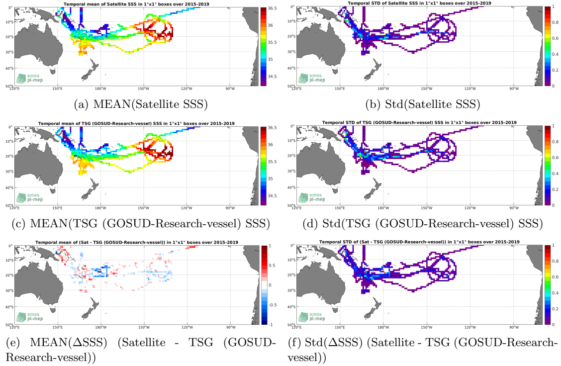
Figure 6: Temporal mean (left) and Std (right) of SSS from SMAP SSS L3 v4 - Monthly (RSS) (top), TSG (GOSUD-Research-vessel) (middle), and of \Delta SSS (Satellite - TSG (GOSUD-Research-vessel)). Only match-up pairs are used to generate these maps.
