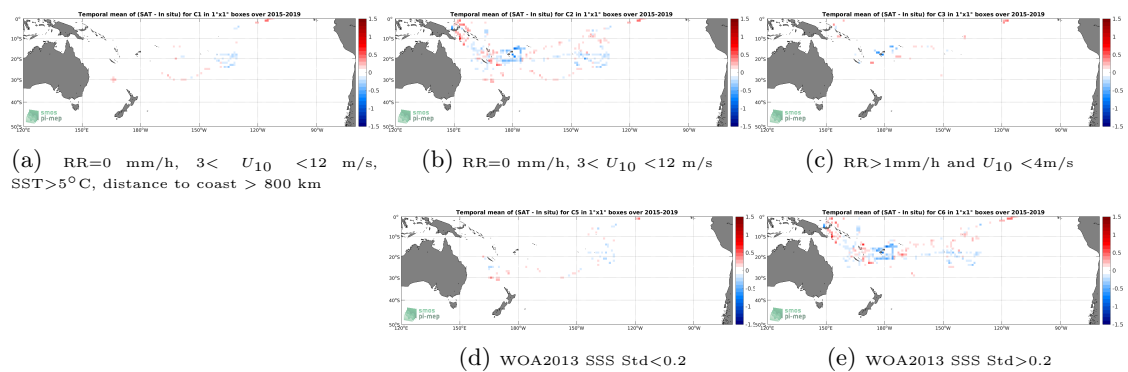
Figure 12: Temporal mean gridded over spatial boxes of size 1^\circ \times 1^\circ of \Delta\text{SSS} (SMAP SSS L3 v4 - Monthly (RSS) - TSG (GOSUD-Research-vessel)) for 5 different subdatasets corresponding to: RR=0 mm/h, 3 < U_{10} < 12 m/s, SST > 5°C, distance to coast > 800 km (a), RR=0 mm/h, 3 < U_{10} < 12 m/s (b), RR > 1mm/h and U_{10} < 4 m/s (c), WOA2013 SSS Std < 0.2 (d), WOA2013 SSS Std > 0.2 (e).
