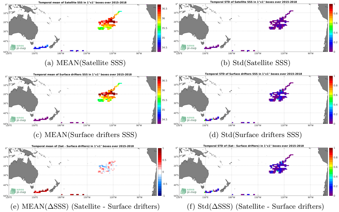
Figure 5: Temporal mean (left) and Std (right) of SSS from SMAP SSS L3 v4 - Monthly (RSS) (top), Surface drifters (middle), and of \Delta SSS (Satellite - Surface drifters). Only match-up pairs are used to generate these maps.
