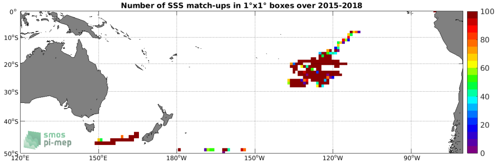
Figure 3: Number of SSS match-ups between Surface drifters SSS and the SMAP SSS L3 v4 - Monthly (RSS) SSS product for the South Pacific Ocean Pi-MEP region over 1^\circ \times 1^\circ boxes and for the full satellite product period.
