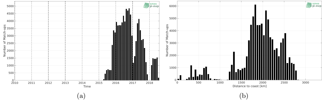
Figure 1: Number of match-ups between Surface drifters and SMAP SSS L3 v4 - Monthly (RSS) SSS as a function of time (a) and as function of the distance to coast (b) over the South Pacific Ocean Pi-MEP region and for the full satellite product period.
