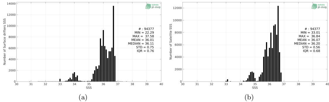
Figure 2: Histograms of SSS from Surface drifters (a) and SMAP SSS L3 v4 - Monthly (RSS) (b) considering all match-up pairs per bins of 0.1 over the South Pacific Ocean Pi-MEP region and for the full satellite product period.
