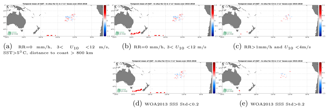
Figure 11: Temporal mean gridded over spatial boxes of size 1^\circ \times 1^\circ of \Delta SSS (SMAP SSS L3 v4 - Monthly (RSS) - Surface drifters) for 5 different subdatasets corresponding to:RR=0 mm/h, 3 < U_{10} < 12 m/s, SST >5^\circ\text{C} , distance to coast > 800 km (a), RR=0 mm/h, 3 < U_{10} < 12 m/s (b), RR >1 mm/h and U_{10} < 4 m/s (c), WOA2013 SSS Std <0.2 (d), WOA2013 SSS Std >0.2 (e).
