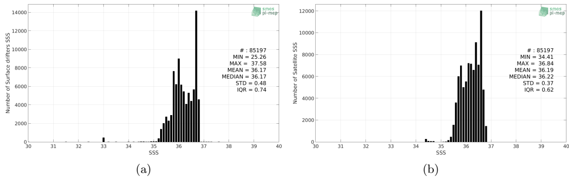
Figure 2: Histograms of SSS from Surface drifters (a) and SMAP-L3-RSS-V4-MONTHLY (b) considering all match-up pairs per bins of 0.1 over the South Pacific Ocean Pi-MEP region and for the full satellite product period.
