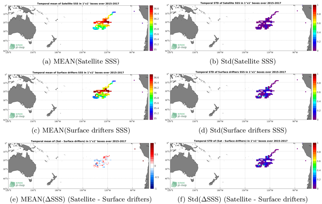
Figure 5: Temporal mean (left) and Std (right) of SSS from SMAP-L3-RSS-V4-MONTHLY (top), Surface drifters (middle), and of \Delta SSS (Satellite - Surface drifters). Only match-up pairs are used to generate these maps.
