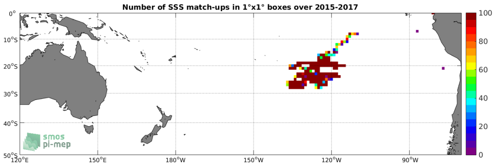
Figure 3: Number of SSS match-ups between Surface drifters SSS and the SMAP-L3-RSS-V4-MONTHLY SSS product for the South Pacific Ocean Pi-MEP region over 1^\circ \times 1^\circ boxes and for the full satellite product period.
