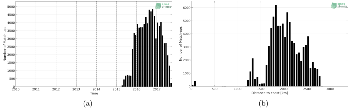
Figure 1: Number of match-ups between Surface drifters and SMAP-L3-RSS-V4-MONTHLY SSS as a function of time (a) and as function of the distance to coast (b) over the South Pacific Ocean Pi-MEP region and for the full satellite product period.
