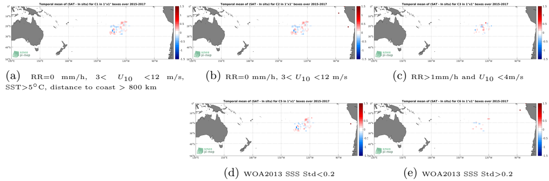
Figure 11: Temporal mean gridded over spatial boxes of size 1^\circ \times 1^\circ of \Delta SSS (SMAP-L3-RSS-V4-MONTHLY - Surface drifters) for 5 different subdatasets corresponding to:RR=0 mm/h, 3 < U_{10} < 12 m/s, SST >5^\circ\text{C} , distance to coast > 800 km (a), RR=0 mm/h, 3 < U_{10} < 12 m/s (b), RR >1 mm/h and U_{10} < 4 m/s (c), WOA2013 SSS Std <0.2 (d), WOA2013 SSS Std >0.2 (e).
