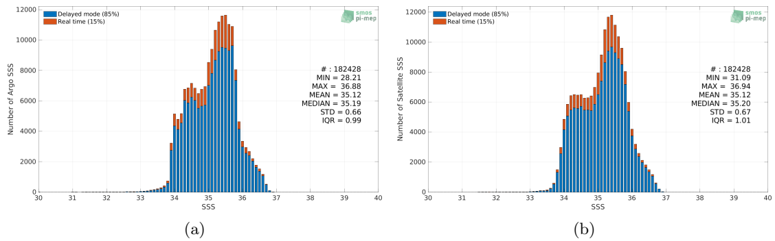
Figure 2: Histograms of SSS from Argo (a) and SMAP SSS L3 v4 - Monthly (RSS) (b) considering all match-up pairs per bins of 0.1 over the South Pacific Ocean Pi-MEP region and for the full satellite product period.
