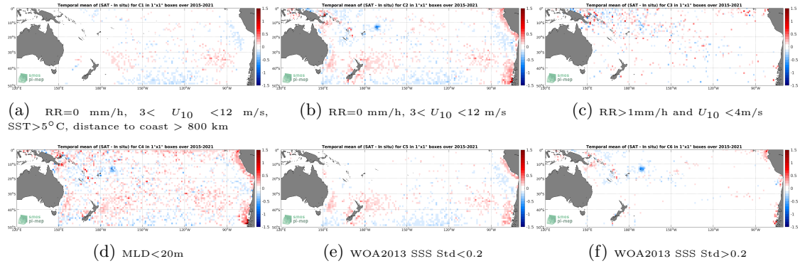
Figure 12: Temporal mean gridded over spatial boxes of size 1^\circ \times 1^\circ of \Delta SSS (SMAP SSS L3 v4 - Monthly (RSS) - Argo) for 6 different subdatasets corresponding to: RR=0 mm/h, 3 < U_{10} < 12 m/s, SST > 5^\circ\text{C} , distance to coast > 800 km (a), RR=0 mm/h, 3 < U_{10} < 12 m/s (b), RR > 1 mm/h and U_{10} < 4 m/s (c), MLD < 20 m (d), WOA2013 SSS Std < 0.2 (e), WOA2013 SSS Std > 0.2 (f).
