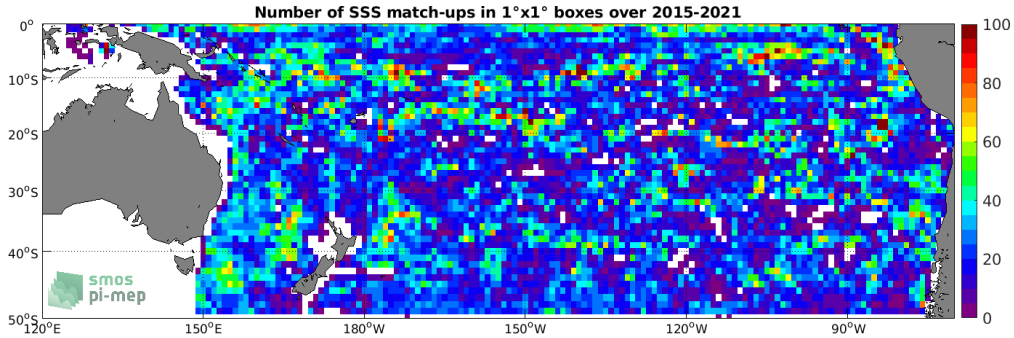
Figure 4: Number of SSS match-ups between Argo SSS and the SMAP SSS L3 v4 - Monthly (RSS) SSS product for the South Pacific Ocean Pi-MEP region over 1^\circ \times 1^\circ boxes and for the full satellite product period.
