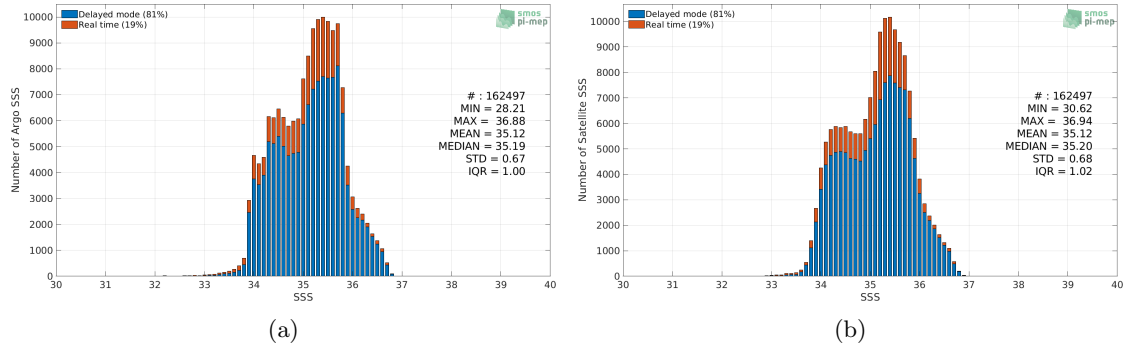
Figure 2: Histograms of SSS from Argo (a) and SMAP SSS L3 v4 - Monthly (RSS) (b) considering all match-up pairs per bins of 0.1 over the South Pacific Ocean Pi-MEP region and for the full satellite product period.
