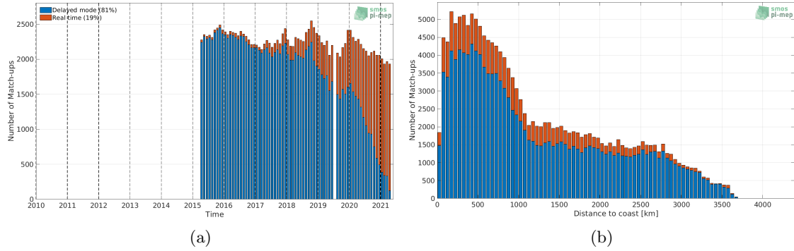
Figure 1: Number of match-ups between Argo and SMAP SSS L3 v4 - Monthly (RSS) SSS as a function of time (a) and as function of the distance to coast (b) over the South Pacific Ocean Pi-MEP region and for the full satellite product period.
