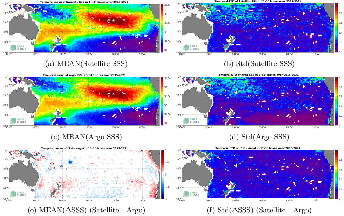
Figure 6: Temporal mean (left) and Std (right) of SSS from SMAP SSS L3 v4 - Monthly (RSS) (top), Argo (middle), and of \Delta SSS (Satellite - Argo). Only match-up pairs are used to generate these maps.
