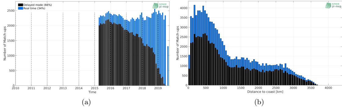
Figure 1: Number of match-ups between Argo and SMAP-L3-RSS-V4-MONTHLY SSS as a function of time (a) and as function of the distance to coast (b) over the South Pacific Ocean Pi-MEP region and for the full satellite product period.
