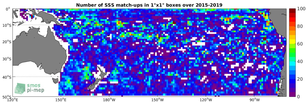
Figure 4: Number of SSS match-ups between Argo SSS and the SMAP-L3-RSS-V4-MONTHLY SSS product for the South Pacific Ocean Pi-MEP region over 1^\circ \times 1^\circ boxes and for the full satellite product period.
