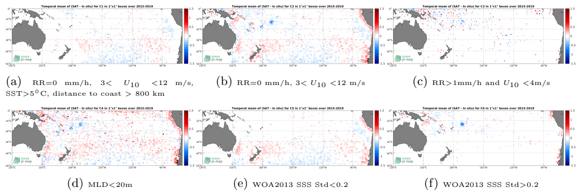
Figure 12: Temporal mean gridded over spatial boxes of size 1^\circ \times 1^\circ of \Delta SSS (SMAP-L3-RSS-V4-MONTHLY - Argo) for 6 different subdatasets corresponding to:RR=0 mm/h, 3 < U_{10} < 12 m/s, SST >5^\circ C, distance to coast > 800 km (a), RR=0 mm/h, 3 < U_{10} < 12 m/s (b), RR >1 mm/h and U_{10} < 4 m/s (c),MLD <20 m (d),WOA2013 SSS Std <0.2 (e),WOA2013 SSS Std >0.2 (f).
