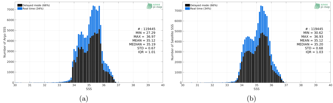
Figure 2: Histograms of SSS from Argo (a) and SMAP-L3-RSS-V4-MONTHLY (b) considering all match-up pairs per bins of 0.1 over the South Pacific Ocean Pi-MEP region and for the full satellite product period.
