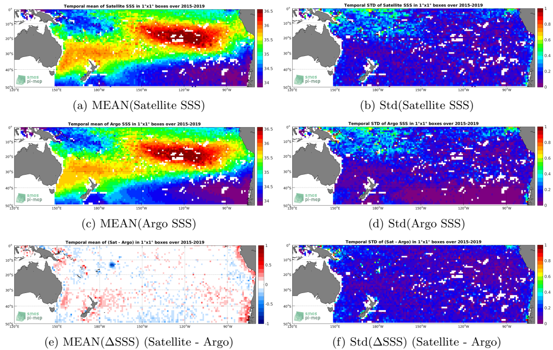
Figure 6: Temporal mean (left) and Std (right) of SSS from SMAP-L3-RSS-V4-MONTHLY (top), Argo (middle), and of \Delta SSS (Satellite - Argo). Only match-up pairs are used to generate these maps.
