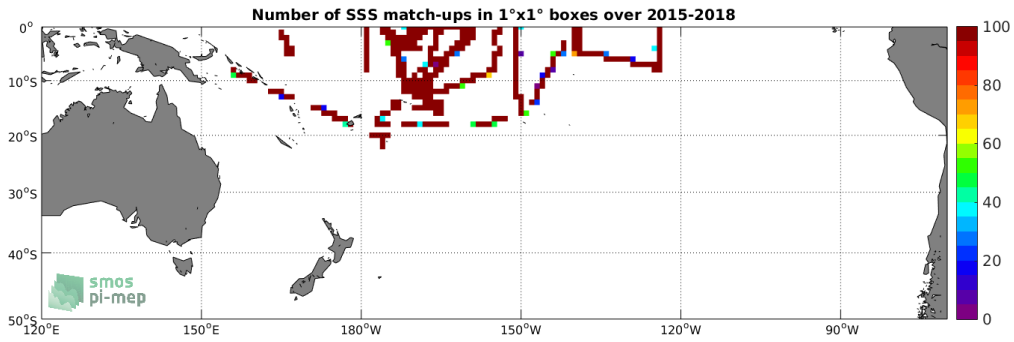
Figure 4: Number of SSS match-ups between TSG-SAMOS SSS and the SMAP-L3-RSS-V3-8DAY-RUNNING-70KM SSS product for the South Pacific Ocean Pi-MEP region over 1^\circ \times 1^\circ boxes and for the full satellite product period.
