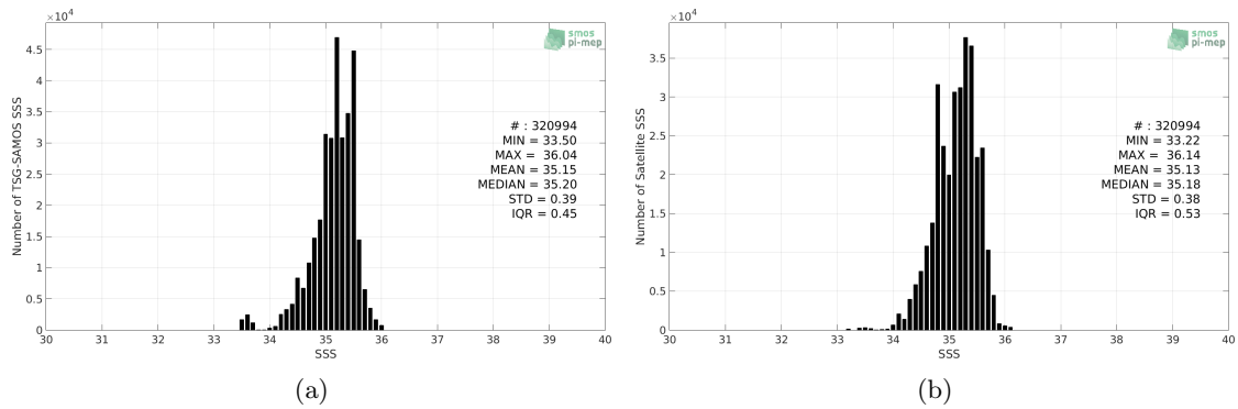
Figure 2: Histograms of SSS from TSG-SAMOS (a) and SMAP-L3-RSS-V3-8DAY-RUNNING-70KM (b) considering all match-up pairs per bins of 0.1 over the South Pacific Ocean Pi-MEP region and for the full satellite product period.
