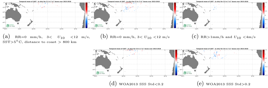
Figure 12: Temporal mean gridded over spatial boxes of size 1^\circ \times 1^\circ of \Delta SSS (SMAP-L3-RSS-V3-8DAY-RUNNING-70KM - TSG-SAMOS) for 5 different subdatasets corresponding to: RR=0 mm/h, 3 < U_{10} < 12 m/s, SST > 5^\circ C , distance to coast > 800 km (a), RR=0 mm/h, 3 < U_{10} < 12 m/s (b), RR > 1 mm/h and U_{10} < 4 m/s (c), WOA2013 SSS Std < 0.2 (d), WOA2013 SSS Std > 0.2 (e).
