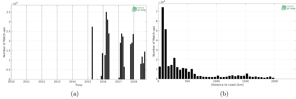
Figure 1: Number of match-ups between TSG-SAMOS and SMAP-L3-RSS-V3-8DAY-RUNNING-70KM SSS as a function of time (a) and as function of the distance to coast (b) over the South Pacific Ocean Pi-MEP region and for the full satellite product period.
