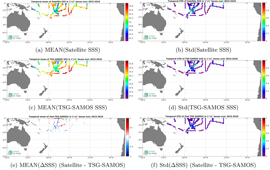
Figure 6: Temporal mean (left) and Std (right) of SSS from SMAP-L3-RSS-V3-8DAY-RUNNING-70KM (top), TSG-SAMOS (middle), and of \Delta SSS (Satellite - TSG-SAMOS). Only match-up pairs are used to generate these maps.
