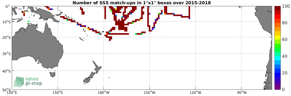
Figure 4: Number of SSS match-ups between TSG-SAMOS SSS and the SMAP-L3-RSS-V3-8DAY-RUNNING-70KM SSS product for the South Pacific Ocean Pi-MEP region over 1°x1° boxes and for the full satellite product period.
