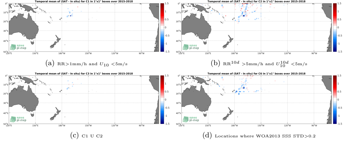
Figure 12: Temporal mean gridded over spatial boxes of size 1^\circ \times 1^\circ of \Delta SSS (SMAP-L3-RSS-V3-8DAY-RUNNING-70KM - TSG-SAMOS) for 4 different subdatasets corresponding to: RR > 1mm/h and U_{10} < 5\text{m/s} (a), RR^{10d} > 5\text{mm/h} and U_{10}^{10d} < 5\text{m/s} (b), C1 U C2 (c), Locations where WOA2013 SSS STD > 0.2 (d).
