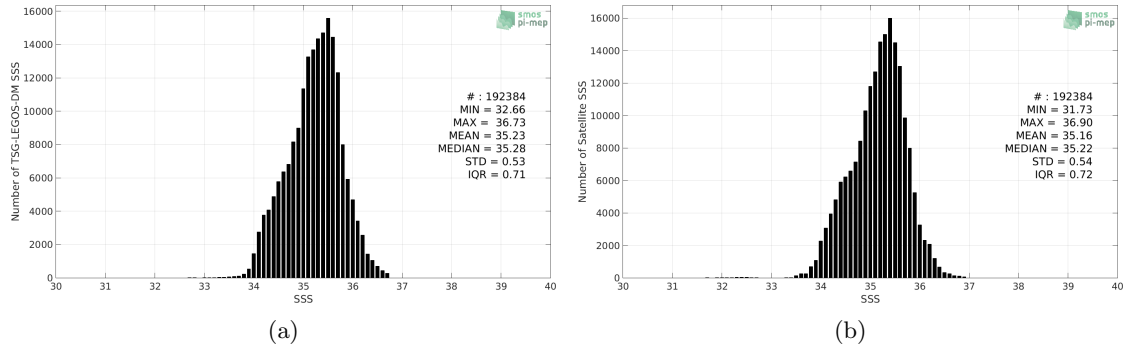
Figure 2: Histograms of SSS from TSG-LEGOS-DM (a) and SMAP-L3-RSS-V3-8DAY-RUNNING-70KM (b) considering all match-up pairs per bins of 0.1 over the South Pacific Ocean Pi-MEP region and for the full satellite product period.
