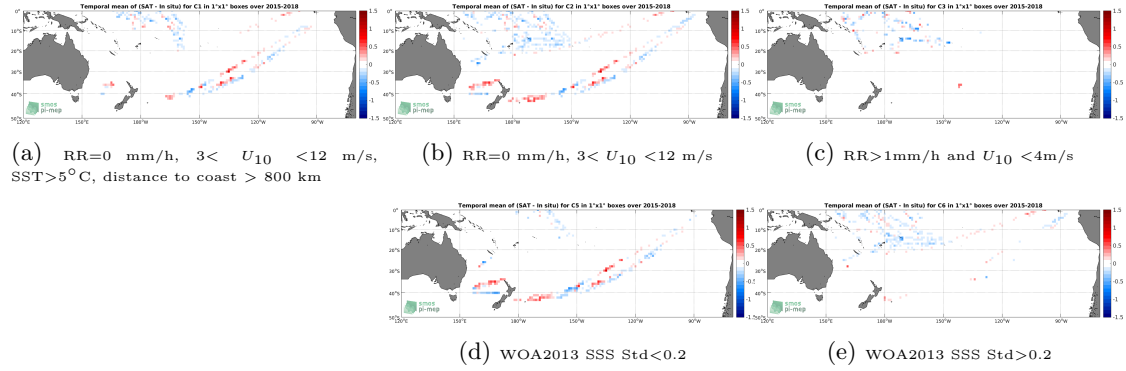
Figure 12: Temporal mean gridded over spatial boxes of size 1^\circ \times 1^\circ of \Delta SSS (SMAP-L3-RSS-V3-8DAY-RUNNING-70KM - TSG-LEGOS-DM) for 5 different subdatasets corresponding to: RR=0 mm/h, 3 < U_{10} < 12 m/s, SST > 5^\circ C , distance to coast > 800 km (a), RR=0 mm/h, 3 < U_{10} < 12 m/s (b), RR > 1 mm/h and U_{10} < 4 m/s (c), WOA2013 SSS Std < 0.2 (d), WOA2013 SSS Std > 0.2 (e).
