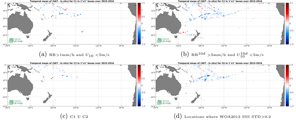
Figure 12: Temporal mean gridded over spatial boxes of size 1^\circ \times 1^\circ of \Delta SSS (SMAP-L3-RSS-V3-8DAY-RUNNING-70KM - TSG-LEGOS-DM) for 4 different subdatasets corresponding to: RR > 1mm/h and U_{10} < 5\text{m/s} (a), RR^{10d} > 5\text{mm/h} and U_{10}^{10d} < 5\text{m/s} (b), C1 U C2 (c), Locations where WOA2013 SSS STD > 0.2 (d).
