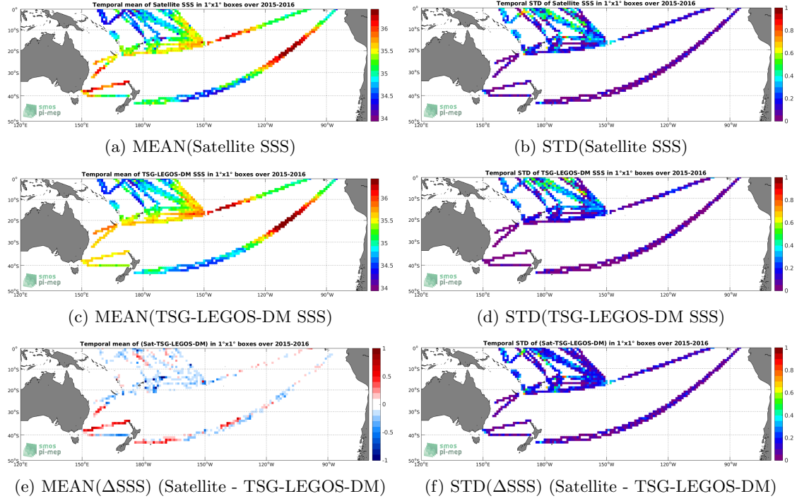
Figure 6: Temporal mean (left) and STD (right) of SSS from SMAP-L3-RSS-V3-8DAY-RUNNING-70KM (top), TSG-LEGOS-DM (middle), and of \Delta SSS (Satellite - TSG-LEGOS-DM). Only match-up pairs are used to generate these maps.
