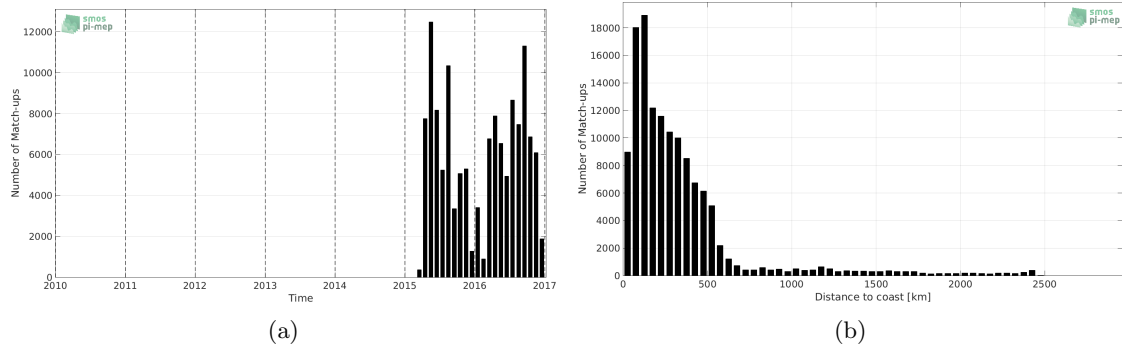
Figure 1: Number of match-ups between TSG-LEGOS-DM and SMAP-L3-RSS-V3-8DAY-RUNNING-70KM SSS as a function of time (a) and as function of the distance to coast (b) over the South Pacific Ocean Pi-MEP region and for the full satellite product period.
