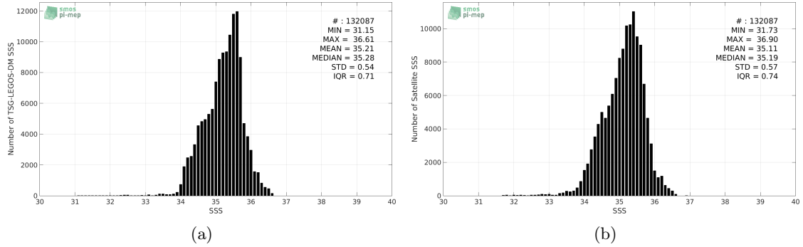
Figure 2: Histograms of SSS from TSG-LEGOS-DM (a) and SMAP-L3-RSS-V3-8DAY-RUNNING-70KM (b) considering all match-up pairs per bins of 0.1 over the South Pacific Ocean Pi-MEP region and for the full satellite product period.
