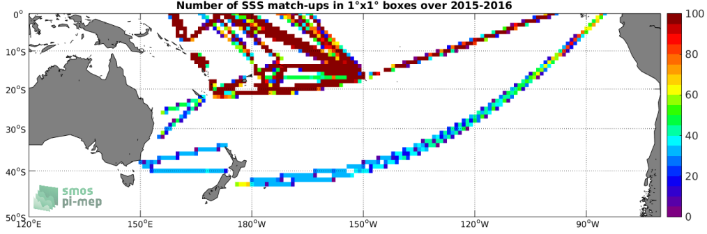
Figure 4: Number of SSS match-ups between TSG-LEGOS-DM SSS and the SMAP-L3-RSS-V3-8DAY-RUNNING-70KM SSS product for the South Pacific Ocean Pi-MEP region over 1^\circ \times 1^\circ boxes and for the full satellite product period.
