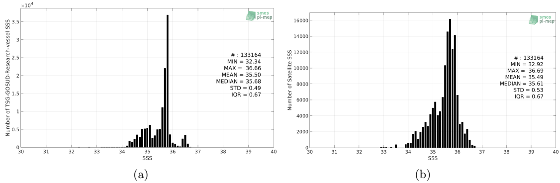
Figure 2: Histograms of SSS from TSG-GOSUD-Research-vessel (a) and SMAP-L3-RSS-V3-8DAY-RUNNING-70KM (b) considering all match-up pairs per bins of 0.1 over the South Pacific Ocean Pi-MEP region and for the full satellite product period.
