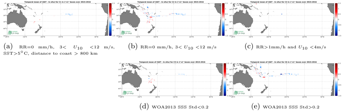
Figure 12: Temporal mean gridded over spatial boxes of size 1^\circ \times 1^\circ of \Delta SSS (SMAP-L3-RSS-V3-8DAY-RUNNING-70KM - TSG-GOSUD-Research-vessel) for 5 different subdatasets corresponding to: RR=0 mm/h, 3 < U_{10} < 12 m/s, SST > 5^\circ C , distance to coast > 800 km (a), RR=0 mm/h, 3 < U_{10} < 12 m/s (b), RR > 1 mm/h and U_{10} < 4 m/s (c), WOA2013 SSS Std < 0.2 (d), WOA2013 SSS Std > 0.2 (e).
