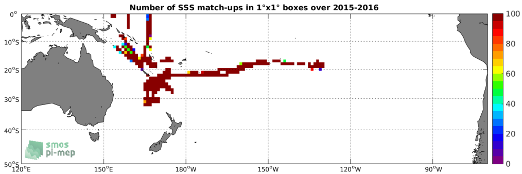
Figure 4: Number of SSS match-ups between TSG-GOSUD-Research-vessel SSS and the SMAP-L3-RSS-V3-8DAY-RUNNING-70KM SSS product for the South Pacific Ocean Pi-MEP region over 1^\circ \times 1^\circ boxes and for the full satellite product period.
