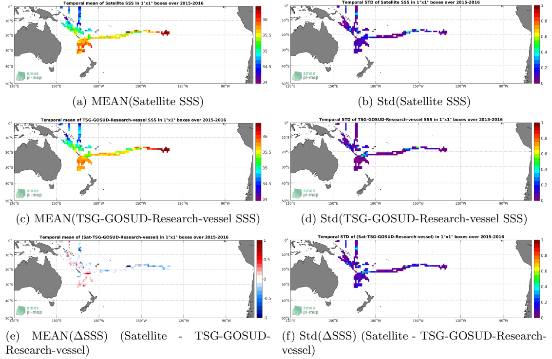
Figure 6: Temporal mean (left) and Std (right) of SSS from SMAP-L3-RSS-V3-8DAY-RUNNING-70KM (top), TSG-GOSUD-Research-vessel (middle), and of \Delta SSS (Satellite - TSG-GOSUD-Research-vessel). Only match-up pairs are used to generate these maps.
