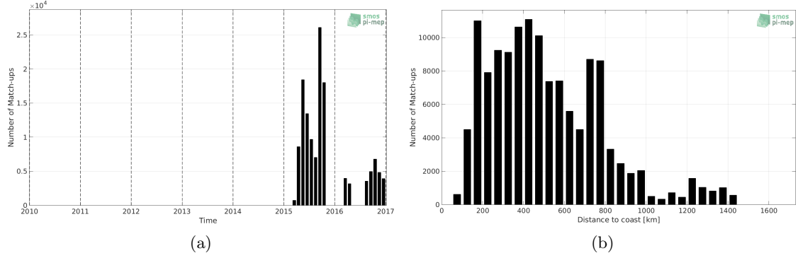
Figure 1: Number of match-ups between TSG-GOSUD-Research-vessel and SMAP-L3-RSS-V3-8DAY-RUNNING-70KM SSS as a function of time (a) and as function of the distance to coast (b) over the South Pacific Ocean Pi-MEP region and for the full satellite product period.
