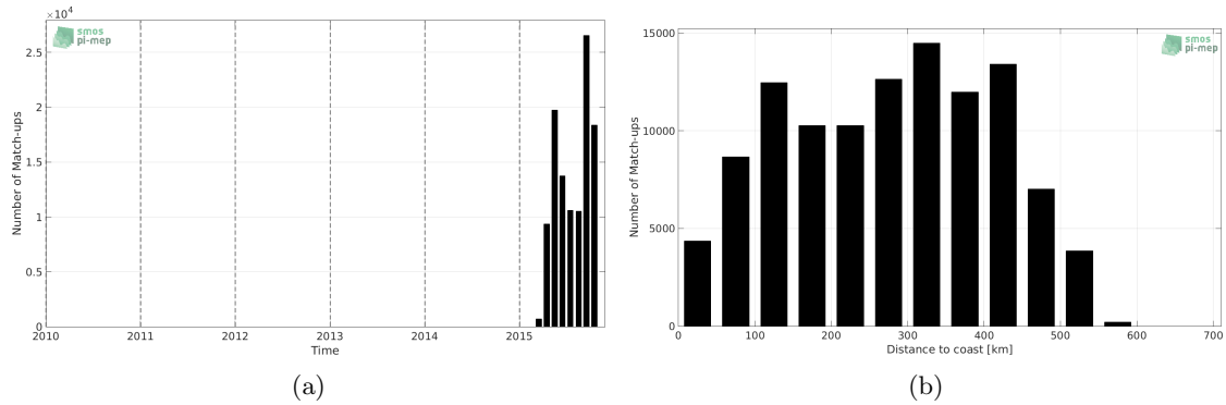
Figure 1: Number of match-ups between TSG-GOSUD-Research-vessel and SMAP-L3-RSS-V3-8DAY-RUNNING-70KM SSS as a function of time (a) and as function of the distance to coast (b) over the South Pacific Ocean Pi-MEP region and for the full satellite product period.
