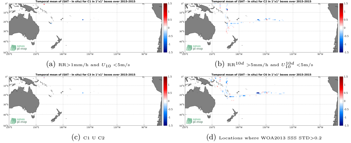
Figure 12: Temporal mean gridded over spatial boxes of size 1^\circ \times 1^\circ of \Delta SSS (SMAP-L3-RSS-V3-8DAY-RUNNING-70KM - TSG-GOSUD-Research-vessel) for 4 different subdatasets corresponding to: RR > 1\text{mm/h} and U_{10} < 5\text{m/s} (a), RR^{10d} > 5\text{mm/h} and U_{10}^{10d} < 5\text{m/s} (b), C1 U C2 (c), Locations where WOA2013 SSS STD > 0.2 (d).
