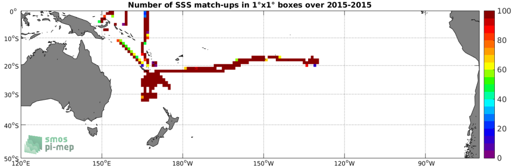
Figure 4: Number of SSS match-ups between TSG-GOSUD-Research-vessel SSS and the SMAP-L3-RSS-V3-8DAY-RUNNING-70KM SSS product for the South Pacific Ocean Pi-MEP region over 1°x1° boxes and for the full satellite product period.
