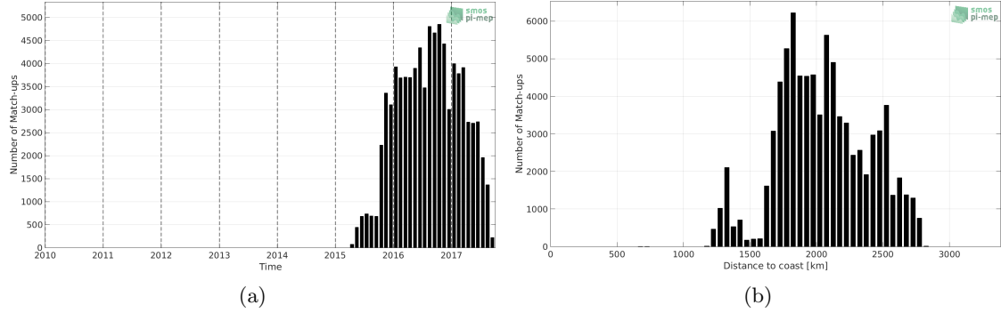
Figure 1: Number of match-ups between Surface drifters and SMAP-L3-RSS-V3-8DAY-RUNNING-70KM SSS as a function of time (a) and as function of the distance to coast (b) over the South Pacific Ocean Pi-MEP region and for the full satellite product period.
