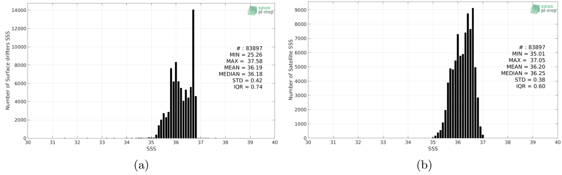
Figure 2: Histograms of SSS from Surface drifters (a) and SMAP-L3-RSS-V3-8DAY-RUNNING-70KM (b) considering all match-up pairs per bins of 0.1 over the South Pacific Ocean Pi-MEP region and for the full satellite product period.
