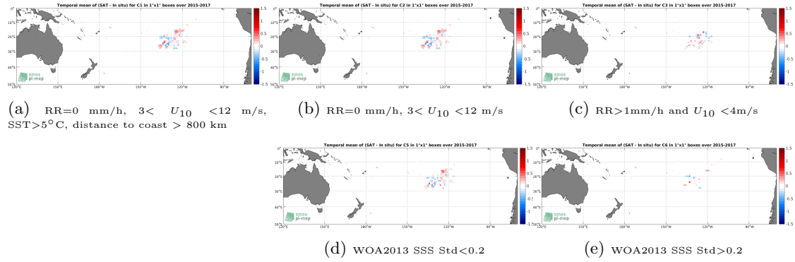
Figure 11: Temporal mean gridded over spatial boxes of size 1^\circ \times 1^\circ of \Delta SSS (SMAP-L3-RSS-V3-8DAY-RUNNING-70KM - Surface drifters) for 5 different subdatasets corresponding to: RR=0 mm/h, 3 < U_{10} < 12 m/s, SST > 5^\circ C, distance to coast > 800 km (a), RR=0 mm/h, 3 < U_{10} < 12 m/s (b), RR > 1 mm/h and U_{10} < 4 m/s (c), WOA2013 SSS Std < 0.2 (d), WOA2013 SSS Std > 0.2 (e).
