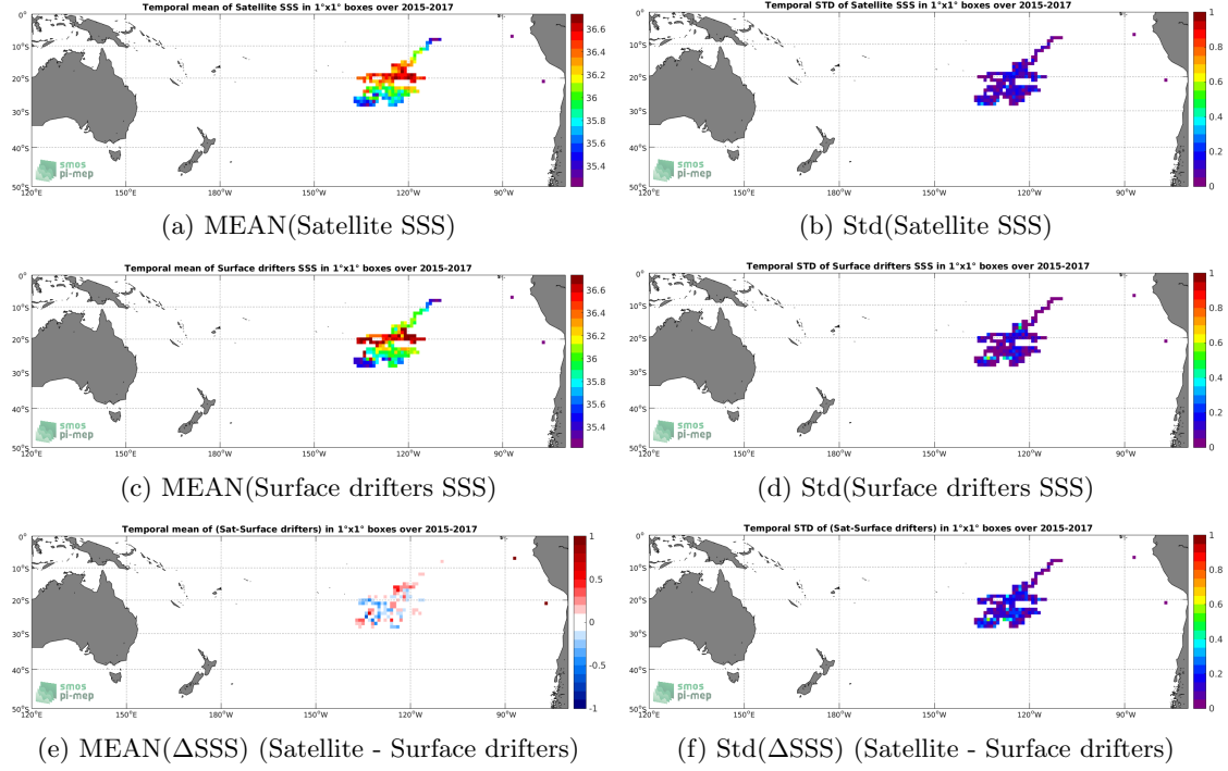
Figure 5: Temporal mean (left) and Std (right) of SSS from SMAP-L3-RSS-V3-8DAY-RUNNING-70KM (top), Surface drifters (middle), and of \Delta SSS (Satellite - Surface drifters). Only match-up pairs are used to generate these maps.
