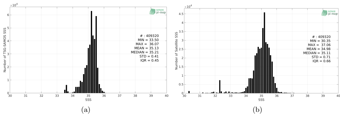
Figure 2: Histograms of SSS from TSG-SAMOS (a) and SMAP-L3-RSS-V3-8DAY-RUNNING-40KM (b) considering all match-up pairs per bins of 0.1 over the South Pacific Ocean Pi-MEP region and for the full satellite product period.
