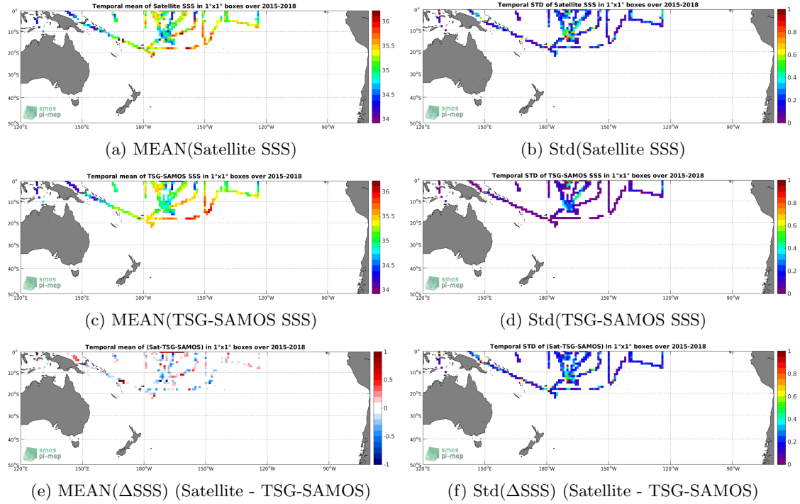
Figure 6: Temporal mean (left) and Std (right) of SSS from SMAP-L3-RSS-V3-8DAY-RUNNING-40KM (top), TSG-SAMOS (middle), and of \Delta SSS (Satellite - TSG-SAMOS). Only match-up pairs are used to generate these maps.
