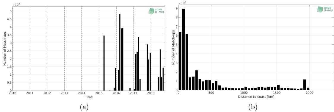
Figure 1: Number of match-ups between TSG-SAMOS and SMAP-L3-RSS-V3-8DAY-RUNNING-40KM SSS as a function of time (a) and as function of the distance to coast (b) over the South Pacific Ocean Pi-MEP region and for the full satellite product period.
