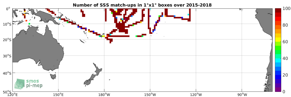
Figure 4: Number of SSS match-ups between TSG-SAMOS SSS and the SMAP-L3-RSS-V3-8DAY-RUNNING-40KM SSS product for the South Pacific Ocean Pi-MEP region over 1^\circ \times 1^\circ boxes and for the full satellite product period.
