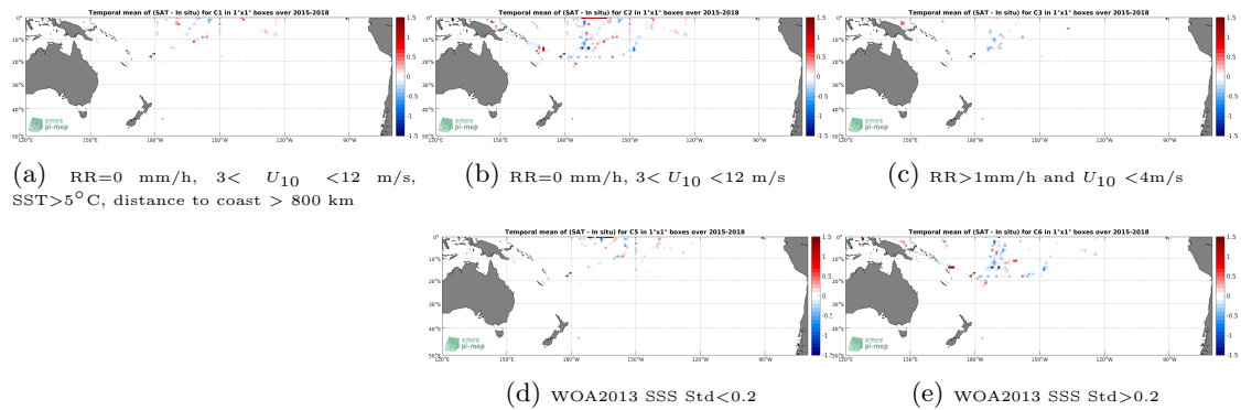
Figure 12: Temporal mean gridded over spatial boxes of size 1^\circ \times 1^\circ of \Delta SSS (SMAP-L3-RSS-V3-8DAY-RUNNING-40KM - TSG-SAMOS) for 5 different subdatasets corresponding to:RR=0 mm/h, 3 < U_{10} < 12 m/s, SST >5^\circ C, distance to coast > 800 km (a), RR=0 mm/h, 3 < U_{10} < 12 m/s (b), RR >1 mm/h and U_{10} < 4 m/s (c), WOA2013 SSS Std <0.2 (d), WOA2013 SSS Std >0.2 (e).
