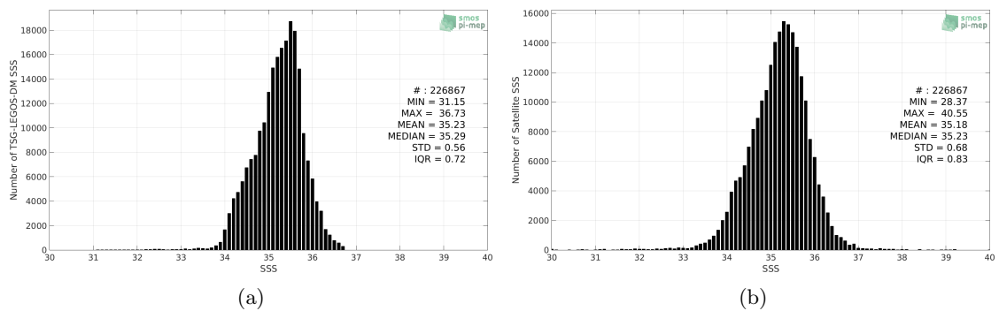
Figure 2: Histograms of SSS from TSG-LEGOS-DM (a) and SMAP-L3-RSS-V3-8DAY-RUNNING-40KM (b) considering all match-up pairs per bins of 0.1 over the South Pacific Ocean Pi-MEP region and for the full satellite product period.
