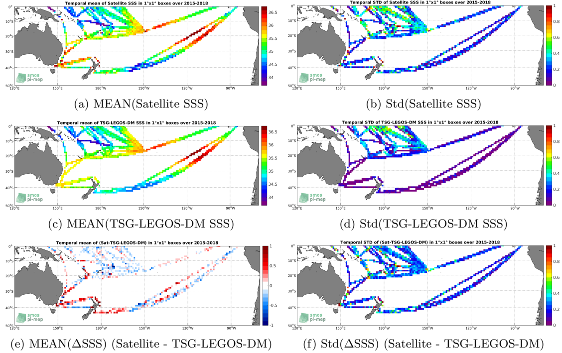
Figure 6: Temporal mean (left) and Std (right) of SSS from SMAP-L3-RSS-V3-8DAY-RUNNING-40KM (top), TSG-LEGOS-DM (middle), and of \Delta SSS (Satellite - TSG-LEGOS-DM). Only match-up pairs are used to generate these maps.
