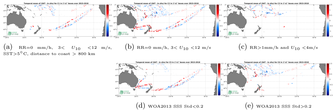
Figure 12: Temporal mean gridded over spatial boxes of size 1^\circ \times 1^\circ of \Delta SSS (SMAP-L3-RSS-V3-8DAY-RUNNING-40KM - TSG-LEGOS-DM) for 5 different subdatasets corresponding to:RR=0 mm/h, 3 < U_{10} < 12 m/s, SST >5^\circ C, distance to coast > 800 km (a), RR=0 mm/h, 3 < U_{10} < 12 m/s (b), RR >1 mm/h and U_{10} < 4 m/s (c), WOA2013 SSS Std <0.2 (d), WOA2013 SSS Std >0.2 (e).
