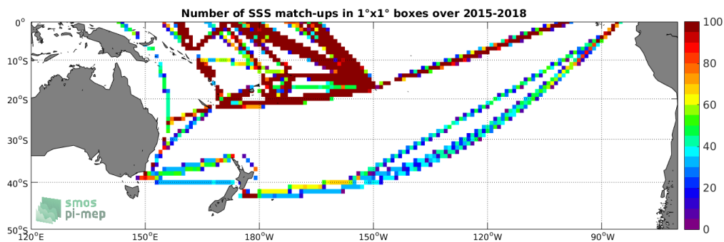
Figure 4: Number of SSS match-ups between TSG-LEGOS-DM SSS and the SMAP-L3-RSS-V3-8DAY-RUNNING-40KM SSS product for the South Pacific Ocean Pi-MEP region over 1^\circ \times 1^\circ boxes and for the full satellite product period.
