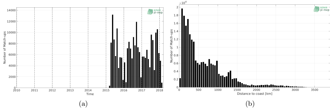
Figure 1: Number of match-ups between TSG-LEGOS-DM and SMAP-L3-RSS-V3-8DAY-RUNNING-40KM SSS as a function of time (a) and as function of the distance to coast (b) over the South Pacific Ocean Pi-MEP region and for the full satellite product period.
