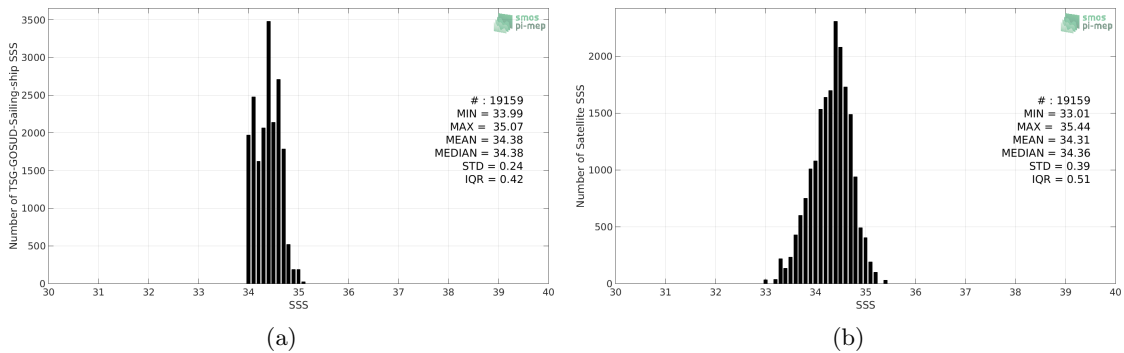
Figure 2: Histograms of SSS from TSG-GOSUD-Sailing-ship (a) and SMAP-L3-RSS-V3-8DAY-RUNNING-40KM (b) considering all match-up pairs per bins of 0.1 over the South Pacific Ocean Pi-MEP region and for the full satellite product period.
