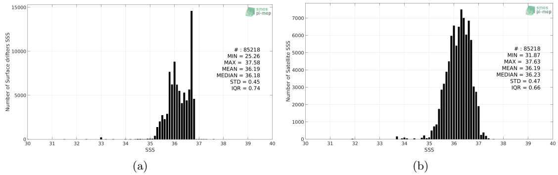
Figure 2: Histograms of SSS from Surface drifters (a) and SMAP-L3-RSS-V3-8DAY-RUNNING-40KM (b) considering all match-up pairs per bins of 0.1 over the South Pacific Ocean Pi-MEP region and for the full satellite product period.
