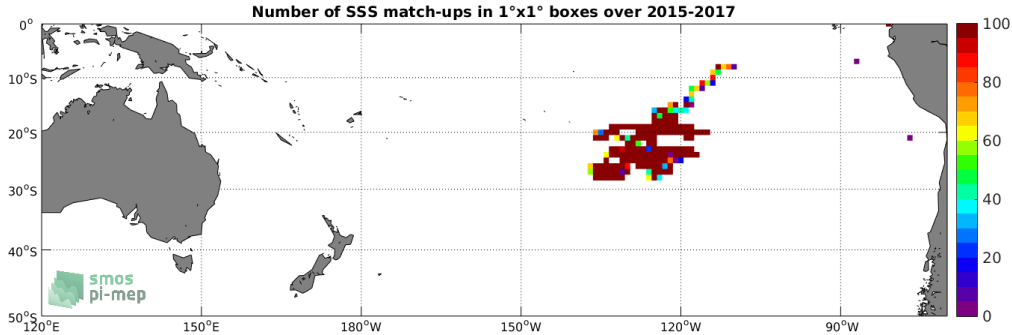
Figure 3: Number of SSS match-ups between Surface drifters SSS and the SMAP-L3-RSS-V3-8DAY-RUNNING-40KM SSS product for the South Pacific Ocean Pi-MEP region over 1^\circ \times 1^\circ boxes and for the full satellite product period.
