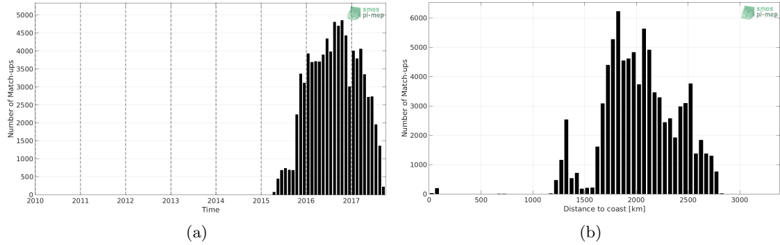
Figure 1: Number of match-ups between Surface drifters and SMAP-L3-RSS-V3-8DAY-RUNNING-40KM SSS as a function of time (a) and as function of the distance to coast (b) over the South Pacific Ocean Pi-MEP region and for the full satellite product period.
