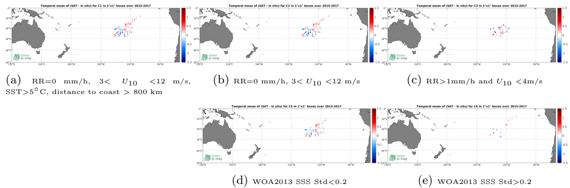
Figure 11: Temporal mean gridded over spatial boxes of size 1^\circ \times 1^\circ of \Delta SSS (SMAP-L3-RSS-V3-8DAY-RUNNING-40KM - Surface drifters) for 5 different subdatasets corresponding to:RR=0 mm/h, 3 < U_{10} < 12 m/s, SST >5^\circ C, distance to coast > 800 km (a), RR=0 mm/h, 3 < U_{10} < 12 m/s (b), RR >1 mm/h and U_{10} < 4 m/s (c), WOA2013 SSS Std <0.2 (d), WOA2013 SSS Std >0.2 (e).
