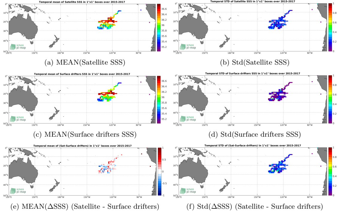
Figure 5: Temporal mean (left) and Std (right) of SSS from SMAP-L3-RSS-V3-8DAY-RUNNING-40KM (top), Surface drifters (middle), and of \Delta SSS (Satellite - Surface drifters). Only match-up pairs are used to generate these maps.
