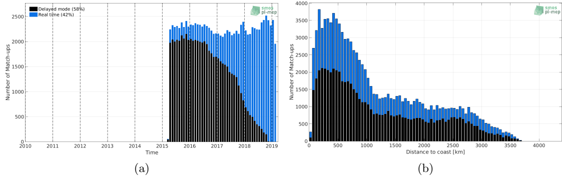
Figure 1: Number of match-ups between Argo and SMAP-L3-RSS-V3-8DAY-RUNNING-40KM SSS as a function of time (a) and as function of the distance to coast (b) over the South Pacific Ocean Pi-MEP region and for the full satellite product period.
