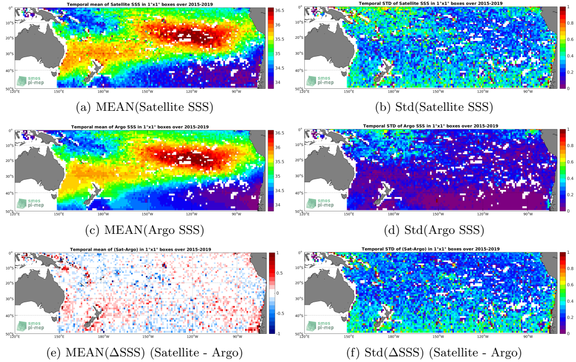
Figure 6: Temporal mean (left) and Std (right) of SSS from SMAP-L3-RSS-V3-8DAY-RUNNING-40KM (top), Argo (middle), and of \Delta SSS (Satellite - Argo). Only match-up pairs are used to generate these maps.
