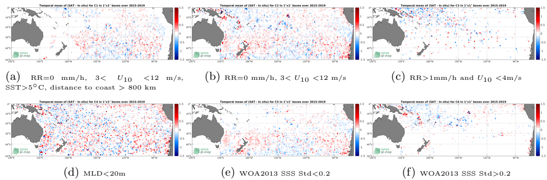
Figure 12: Temporal mean gridded over spatial boxes of size 1^\circ \times 1^\circ of \Delta SSS (SMAP-L3-RSS-V3-8DAY-RUNNING-40KM - Argo) for 6 different subdatasets corresponding to: RR=0 mm/h, 3 < U_{10} < 12 m/s, SST > 5^\circ\text{C} , distance to coast > 800 km (a), RR=0 mm/h, 3 < U_{10} < 12 m/s (b), RR > 1 mm/h and U_{10} < 4 m/s (c), MLD < 20 m (d), WOA2013 SSS Std < 0.2 (e), WOA2013 SSS Std > 0.2 (f).
