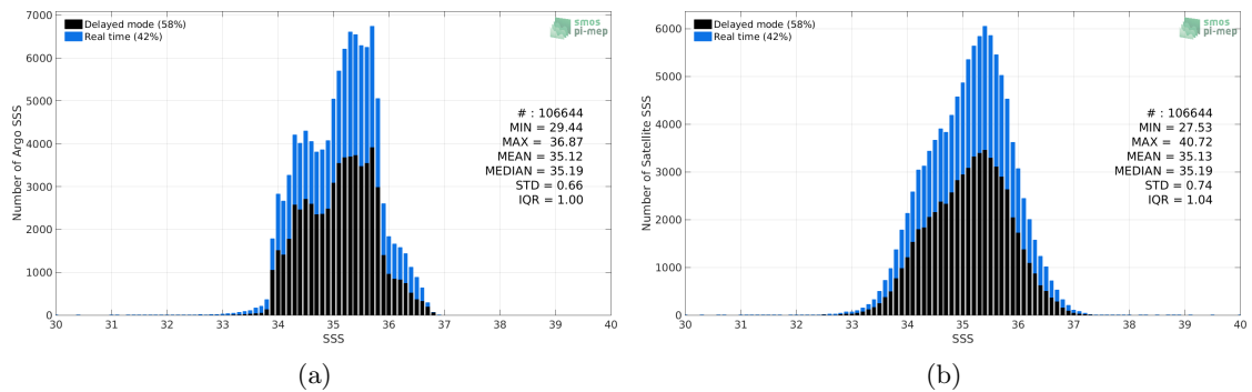
Figure 2: Histograms of SSS from Argo (a) and SMAP-L3-RSS-V3-8DAY-RUNNING-40KM (b) considering all match-up pairs per bins of 0.1 over the South Pacific Ocean Pi-MEP region and for the full satellite product period.
