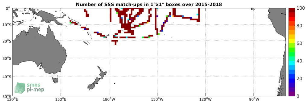
Figure 4: Number of SSS match-ups between TSG-SAMOS SSS and the SMAP-L3-RSS-V3-MONTHLY-70KM SSS product for the South Pacific Ocean Pi-MEP region over 1°x1° boxes and for the full satellite product period.
