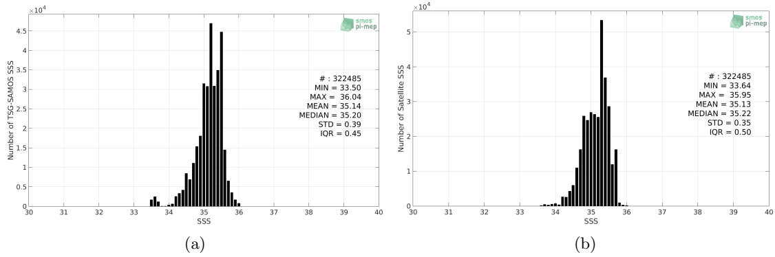
Figure 2: Histograms of SSS from TSG-SAMOS (a) and SMAP-L3-RSS-V3-MONTHLY-70KM (b) considering all match-up pairs per bins of 0.1 over the South Pacific Ocean Pi-MEP region and for the full satellite product period.
