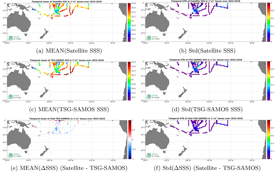
Figure 6: Temporal mean (left) and Std (right) of SSS from SMAP-L3-RSS-V3-MONTHLY-70KM (top), TSG-SAMOS (middle), and of \Delta SSS (Satellite - TSG-SAMOS). Only match-up pairs are used to generate these maps.
