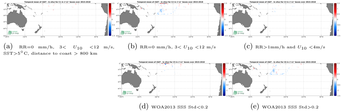
Figure 12: Temporal mean gridded over spatial boxes of size 1^\circ \times 1^\circ of \Delta SSS (SMAP-L3-RSS-V3-MONTHLY-70KM - TSG-SAMOS) for 5 different subdatasets corresponding to: RR=0 mm/h, 3 < U_{10} < 12 m/s, SST > 5^\circ\text{C} , distance to coast > 800 km (a), RR=0 mm/h, 3 < U_{10} < 12 m/s (b), RR > 1 mm/h and U_{10} < 4 m/s (c), WOA2013 SSS Std < 0.2 (d), WOA2013 SSS Std > 0.2 (e).
