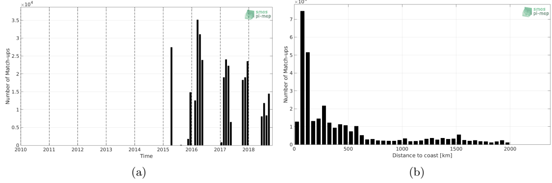
Figure 1: Number of match-ups between TSG-SAMOS and SMAP-L3-RSS-V3-MONTHLY-70KM SSS as a function of time (a) and as function of the distance to coast (b) over the South Pacific Ocean Pi-MEP region and for the full satellite product period.
