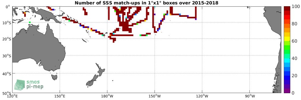
Figure 4: Number of SSS match-ups between TSG-SAMOS SSS and the SMAP-L3-RSS-V3-MONTHLY-70KM SSS product for the South Pacific Ocean Pi-MEP region over 1^\circ \times 1^\circ boxes and for the full satellite product period.
