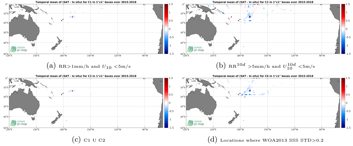
Figure 12: Temporal mean gridded over spatial boxes of size 1^\circ \times 1^\circ of \Delta SSS (SMAP-L3-RSS-V3-MONTHLY-70KM - TSG-SAMOS) for 4 different subdatasets corresponding to: RR > 1\text{mm/h} and U_{10} < 5\text{m/s} (a), RR^{10d} > 5\text{mm/h} and U_{10}^{10d} < 5\text{m/s} (b), C1 U C2 (c), Locations where WOA2013 SSS STD > 0.2 (d).
