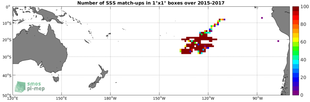
Figure 3: Number of SSS match-ups between Surface drifters SSS and the SMAP-L3-RSS-V3-MONTHLY-70KM SSS product for the South Pacific Ocean Pi-MEP region over 1°x1° boxes and for the full satellite product period.
