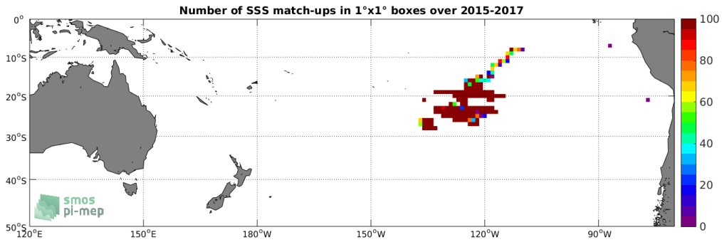
Figure 3: Number of SSS match-ups between Surface drifters SSS and the SMAP-L3-RSS-V3-MONTHLY-70KM SSS product for the South Pacific Ocean Pi-MEP region over 1^\circ \times 1^\circ boxes and for the full satellite product period.
