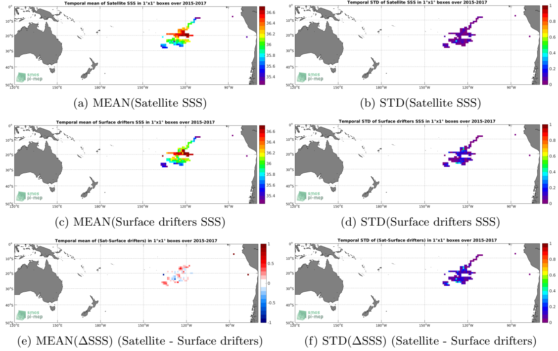
Figure 5: Temporal mean (left) and STD (right) of SSS from SMAP-L3-RSS-V3-MONTHLY-70KM (top), Surface drifters (middle), and of \Delta SSS (Satellite - Surface drifters). Only match-up pairs are used to generate these maps.
