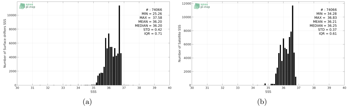
Figure 2: Histograms of SSS from Surface drifters (a) and SMAP-L3-RSS-V3-MONTHLY-70KM (b) considering all match-up pairs per bins of 0.1 over the South Pacific Ocean Pi-MEP region and for the full satellite product period.
