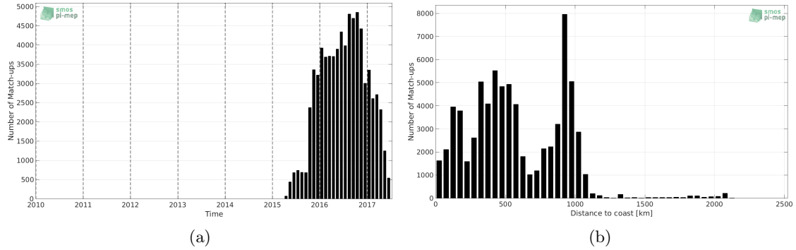
Figure 1: Number of match-ups between Surface drifters and SMAP-L3-RSS-V3-MONTHLY-70KM SSS as a function of time (a) and as function of the distance to coast (b) over the South Pacific Ocean Pi-MEP region and for the full satellite product period.
