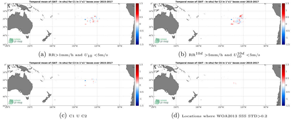
Figure 11: Temporal mean gridded over spatial boxes of size 1^\circ \times 1^\circ of \Delta SSS (SMAP-L3-RSS-V3-MONTHLY-70KM - Surface drifters) for 4 different subdatasets corresponding to: RR > 1mm/h and U_{10} < 5\text{m/s} (a), RR^{10d} > 5\text{mm/h} and U_{10}^{10d} < 5\text{m/s} (b), C1 U C2 (c), Locations where WOA2013 SSS STD > 0.2 (d).
