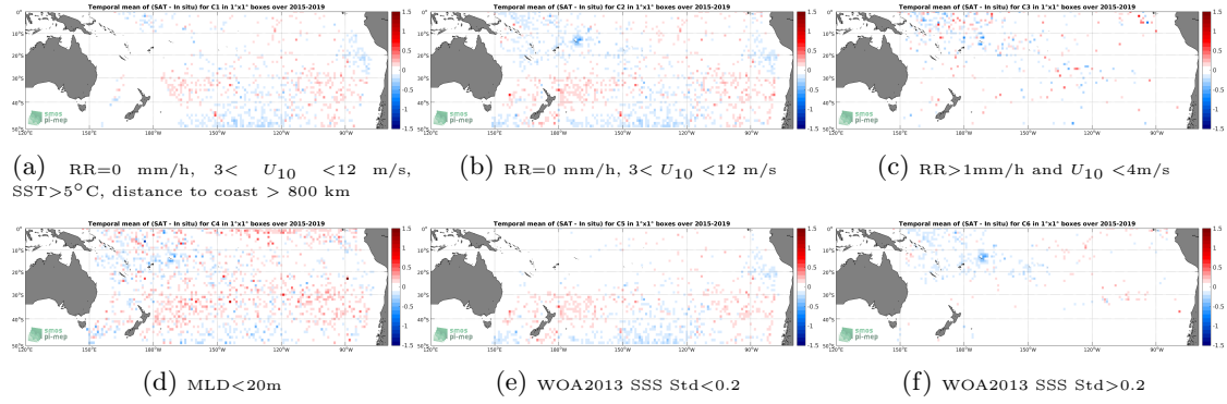
Figure 12: Temporal mean gridded over spatial boxes of size 1^\circ \times 1^\circ of \Delta SSS (SMAP-L3-RSS-V3-MONTHLY-70KM - Argo) for 6 different subdatasets corresponding to: RR=0 mm/h, 3 < U_{10} < 12 m/s, SST > 5^\circ\text{C} , distance to coast > 800 km (a), RR=0 mm/h, 3 < U_{10} < 12 m/s (b), RR > 1 mm/h and U_{10} < 4 m/s (c), MLD < 20 m (d), WOA2013 SSS Std < 0.2 (e), WOA2013 SSS Std > 0.2 (f).
