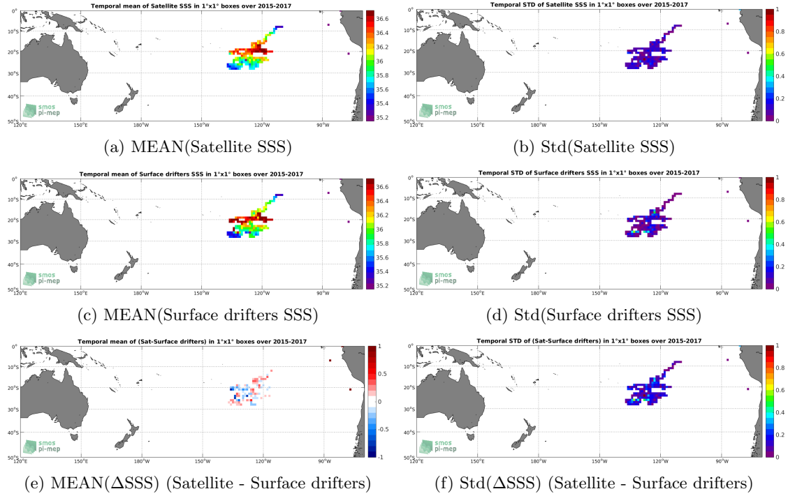
Figure 5: Temporal mean (left) and Std (right) of SSS from SMAP-L3-RSS-V3-MONTHLY-0.25DEG-40KM (top), Surface drifters (middle), and of \Delta SSS (Satellite - Surface drifters). Only match-up pairs are used to generate these maps.
