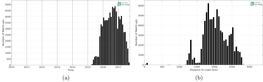
Figure 1: Number of match-ups between Surface drifters and SMAP-L3-RSS-V3-MONTHLY-0.25DEG-40KM SSS as a function of time (a) and as function of the distance to coast (b) over the South Pacific Ocean Pi-MEP region and for the full satellite product period.
