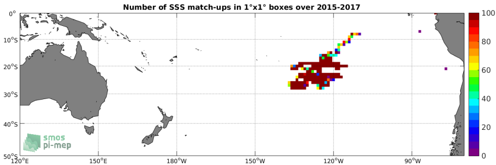
Figure 3: Number of SSS match-ups between Surface drifters SSS and the SMAP-L3-RSS-V3-MONTHLY-0.25DEG-40KM SSS product for the South Pacific Ocean Pi-MEP region over 1^\circ \times 1^\circ boxes and for the full satellite product period.
