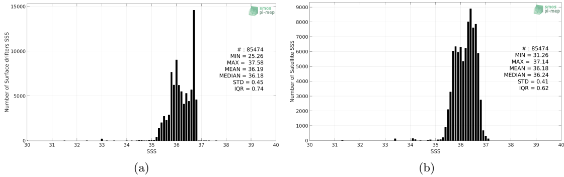
Figure 2: Histograms of SSS from Surface drifters (a) and SMAP-L3-RSS-V3-MONTHLY-0.25DEG-40KM (b) considering all match-up pairs per bins of 0.1 over the South Pacific Ocean Pi-MEP region and for the full satellite product period.
