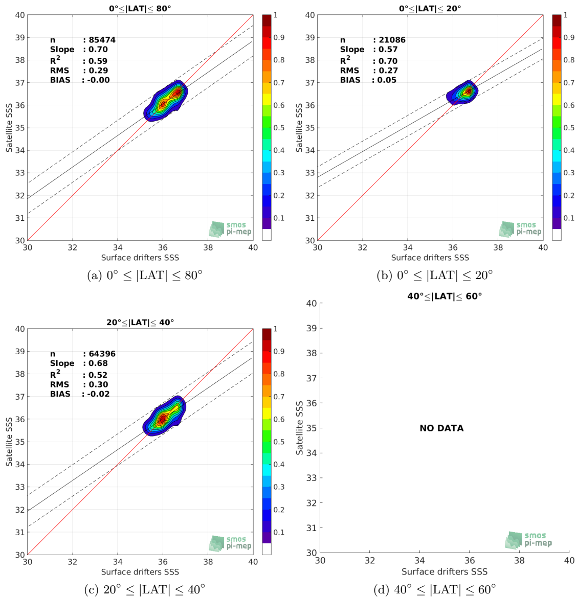
Figure 8: Contour maps of the concentration of SMAP-L3-RSS-V3-MONTHLY-0.25DEG-40KM SSS (y-axis) versus Surface drifters SSS (x-axis) at match-up pairs for different latitude bands. For each plot, the red line shows x=y . The black thin and dashed lines indicate a linear fit through the data cloud and the \pm 95\% confidence levels, respectively. The number match-up pairs n , the slope and R^2 coefficient of the linear fit, the root mean square (RMS) and the mean bias between satellite and in situ data are indicated for each latitude band in each plots.
