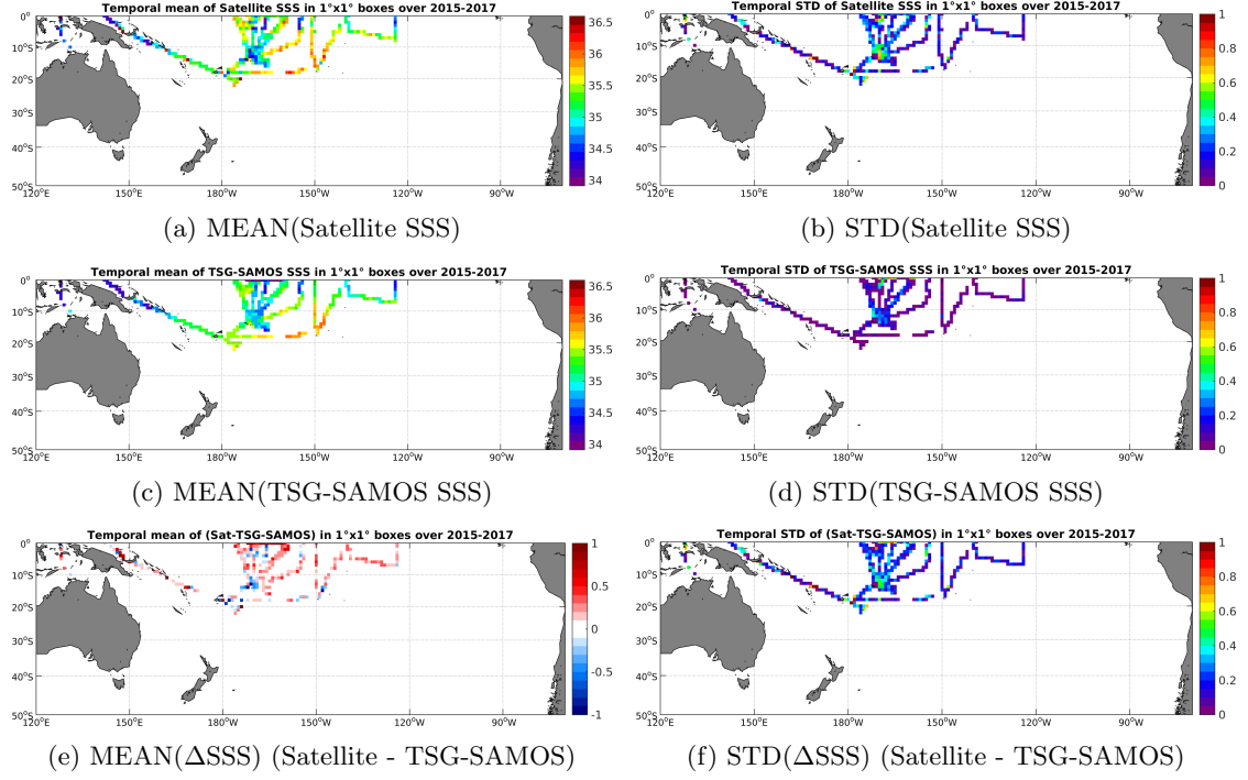
Figure 6: Temporal mean (left) and STD (right) of SSS from SMAP-L3-RSS-V2-8DAY-RUNNING-40KM (top), TSG-SAMOS (middle), and of \Delta SSS (Satellite - TSG-SAMOS). Only match-up pairs are used to generate these maps.
