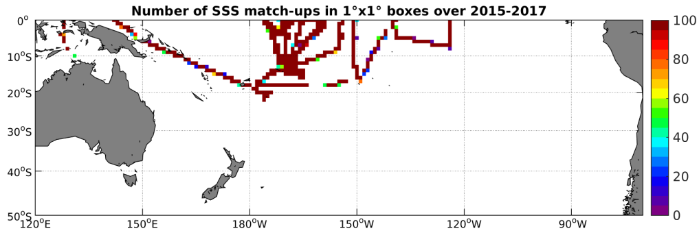
Figure 4: Number of SSS match-ups between TSG-SAMOS SSS and the SMAP-L3-RSS-V2-8DAY-RUNNING-40KM SSS product for the South Pacific Ocean Pi-MEP region over 1^\circ \times 1^\circ boxes and for the full satellite product period.
