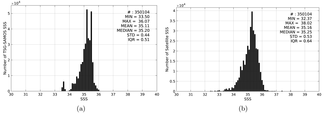
Figure 2: Histograms of SSS from TSG-SAMOS (a) and SMAP-L3-RSS-V2-8DAY-RUNNING-40KM (b) considering all match-up pairs per bins of 0.1 over the South Pacific Ocean Pi-MEP region and for the full satellite product period.
