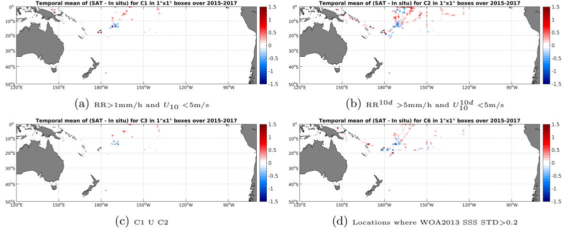
Figure 12: Temporal mean gridded over spatial boxes of size 1^\circ \times 1^\circ of \Delta SSS (SMAP-L3-RSS-V2-8DAY-RUNNING-40KM - TSG-SAMOS) for 4 different subdatasets corresponding to: RR > 1 mm/h and U_{10} < 5 m/s (a), RR^{10d} > 5 mm/h and U_{10}^{10d} < 5 m/s (b), C1 U C2 (c), Locations where WOA2013 SSS STD > 0.2 (d).
