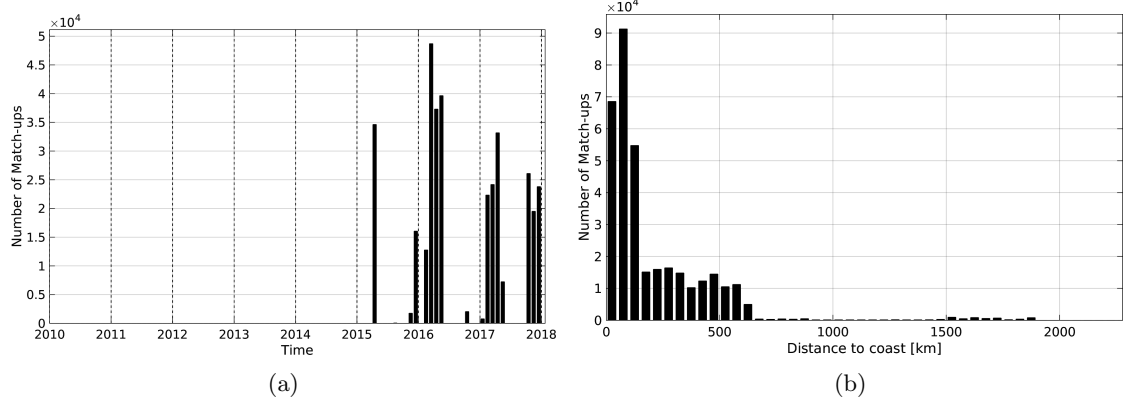
Figure 1: Number of match-ups between TSG-SAMOS and SMAP-L3-RSS-V2-8DAY-RUNNING-40KM SSS as a function of time (a) and as function of the distance to coast (b) over the South Pacific Ocean Pi-MEP region and for the full satellite product period.
