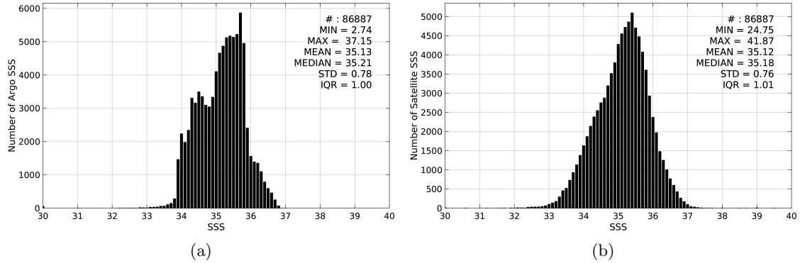
Figure 2: Histograms of SSS from Argo (a) and SMAP-L3-RSS-V2-8DAY-RUNNING-40KM (b) considering all match-up pairs per bins of 0.1 over the South Pacific Ocean Pi-MEP region and for the full satellite product period.
