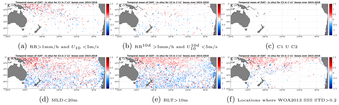
Figure 12: Temporal mean gridded over spatial boxes of size 1^\circ \times 1^\circ of \Delta SSS (SMAP-L3-RSS-V2-8DAY-RUNNING-40KM - Argo) for 6 different subdatasets corresponding to: RR > 1\text{mm/h} and U_{10} < 5\text{m/s} (a), RR^{10d} > 5\text{mm/h} and U_{10}^{10d} < 5\text{m/s} (b), C1 U C2 (c), MLD < 20\text{m} (d), BLT > 10\text{m} (e), Locations where WOA2013 SSS STD > 0.2 (f).
