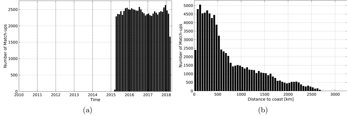
Figure 1: Number of match-ups between Argo and SMAP-L3-RSS-V2-8DAY-RUNNING-40KM SSS as a function of time (a) and as function of the distance to coast (b) over the South Pacific Ocean Pi-MEP region and for the full satellite product period.
