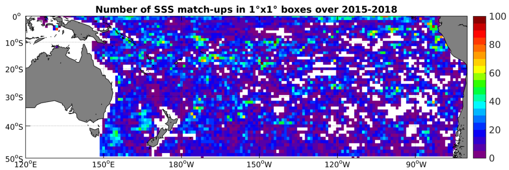
Figure 4: Number of SSS match-ups between Argo SSS and the SMAP-L3-RSS-V2-8DAY-RUNNING-40KM SSS product for the South Pacific Ocean Pi-MEP region over 1^\circ \times 1^\circ boxes and for the full satellite product period.
