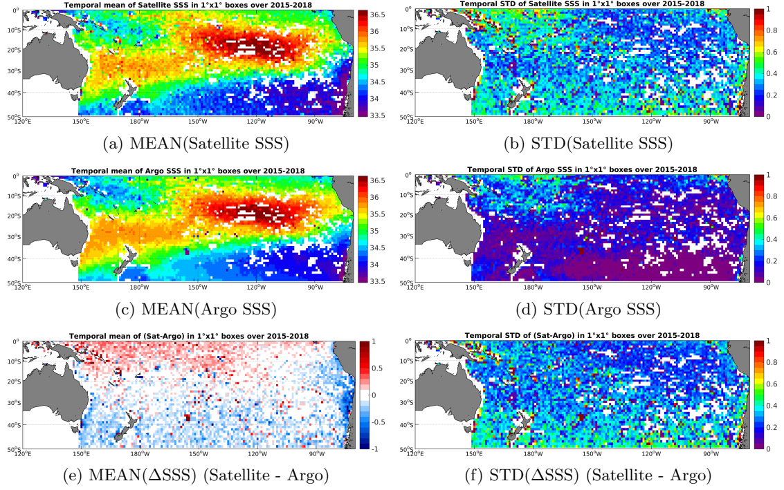
Figure 6: Temporal mean (left) and STD (right) of SSS from SMAP-L3-RSS-V2-8DAY-RUNNING-40KM (top), Argo (middle), and of \Delta SSS (Satellite - Argo). Only match-up pairs are used to generate these maps.
