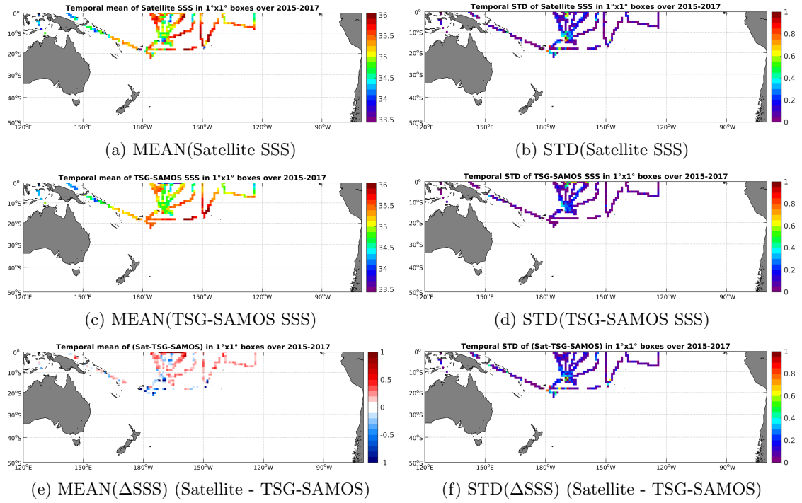
Figure 6: Temporal mean (left) and STD (right) of SSS from SMAP-L3-RSS-V2-8DAY-RUNNING-70KM (top), TSG-SAMOS (middle), and of \Delta SSS (Satellite - TSG-SAMOS). Only match-up pairs are used to generate these maps.
