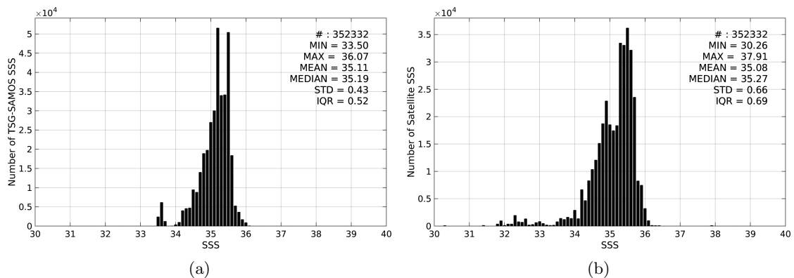
Figure 2: Histograms of SSS from TSG-SAMOS (a) and SMAP-L3-RSS-V2-8DAY-RUNNING-70KM (b) considering all match-up pairs per bins of 0.1 over the South Pacific Ocean Pi-MEP region and for the full satellite product period.
