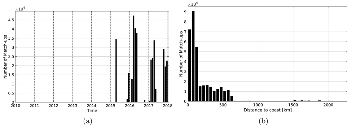
Figure 1: Number of match-ups between TSG-SAMOS and SMAP-L3-RSS-V2-8DAY-RUNNING-70KM SSS as a function of time (a) and as function of the distance to coast (b) over the South Pacific Ocean Pi-MEP region and for the full satellite product period.
