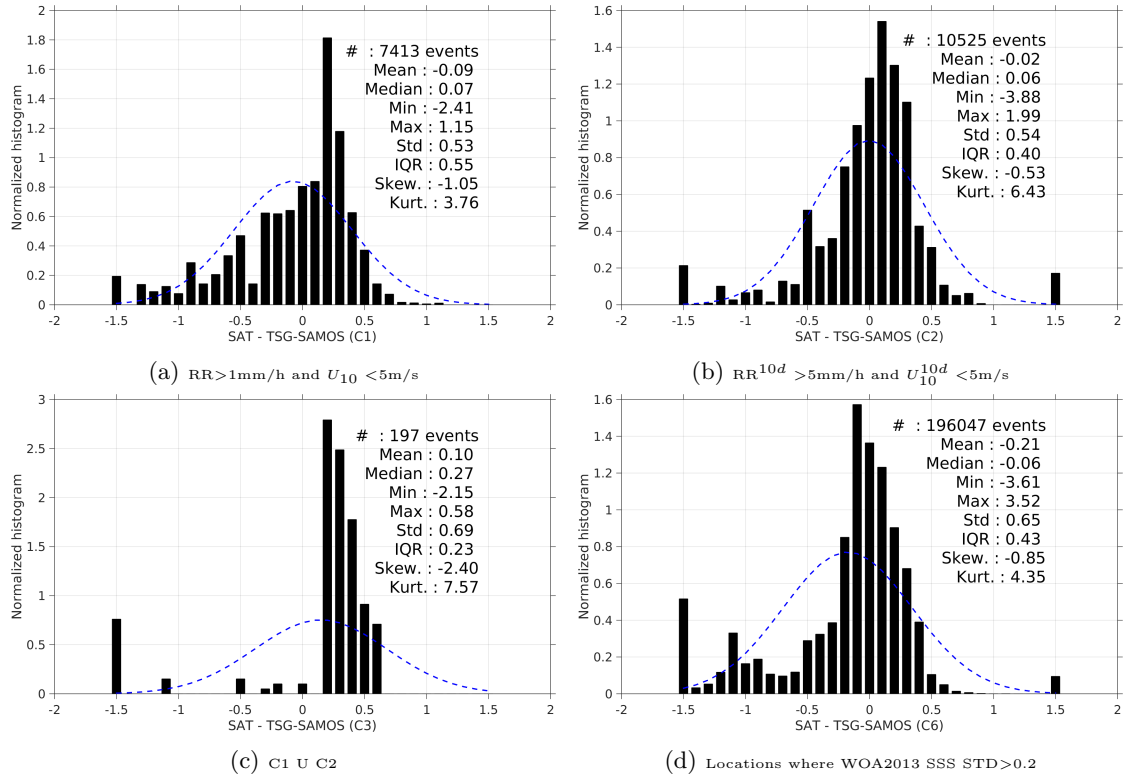
Figure 13: Normalized histogram of \Delta\text{SSS} (SMAP-L3-RSS-V2-8DAY-RUNNING-70KM - TSG-SAMOS) for 6 different subdatasets corresponding to: \text{RR} > 1\text{mm/h} and U_{10} < 5\text{m/s} (a), \text{RR}^{10d} > 5\text{mm/h} and U_{10}^{10d} < 5\text{m/s} (b), C1 U C2 (c), Locations where WOA2013 SSS STD > 0.2 (d).
