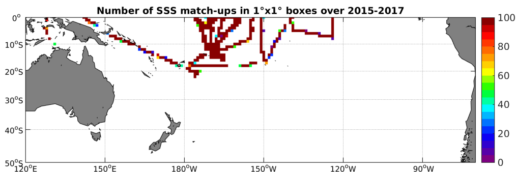
Figure 4: Number of SSS match-ups between TSG-SAMOS SSS and the SMAP-L3-RSS-V2-8DAY-RUNNING-70KM SSS product for the South Pacific Ocean Pi-MEP region over 1^\circ \times 1^\circ boxes and for the full satellite product period.
