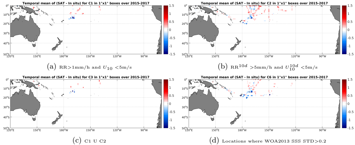
Figure 12: Temporal mean gridded over spatial boxes of size 1^\circ \times 1^\circ of \Delta SSS (SMAP-L3-RSS-V2-8DAY-RUNNING-70KM - TSG-SAMOS) for 4 different subdatasets corresponding to: RR > 1\text{mm/h} and U_{10} < 5\text{m/s} (a), RR^{10d} > 5\text{mm/h} and U_{10}^{10d} < 5\text{m/s} (b), C1 U C2 (c), Locations where WOA2013 SSS STD > 0.2 (d).
