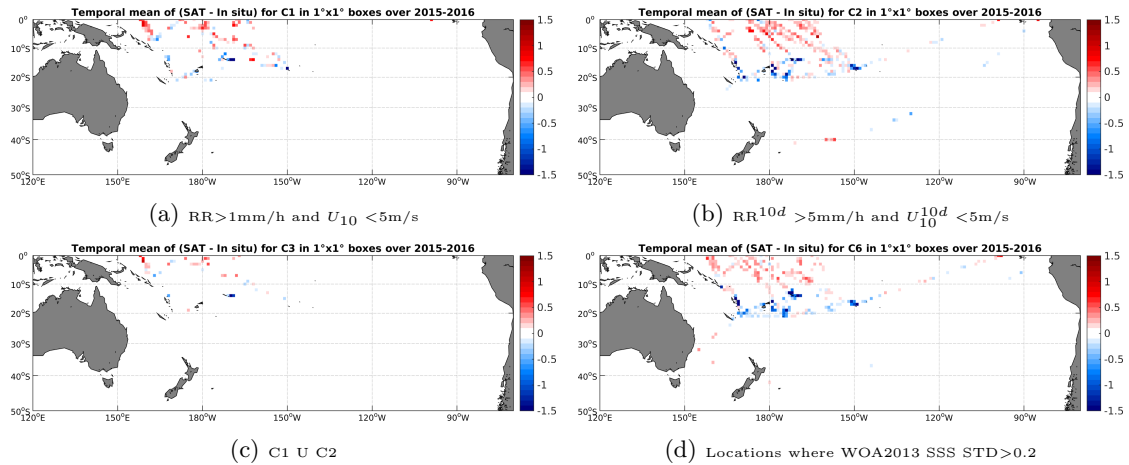
Figure 12: Temporal mean gridded over spatial boxes of size 1^\circ \times 1^\circ of \Delta SSS (SMAP-L3-RSS-V2-8DAY-RUNNING-70KM - TSG-LEGOS-DM) for 4 different subdatasets corresponding to: RR > 1\text{mm/h} and U_{10} < 5\text{m/s} (a), RR^{10d} > 5\text{mm/h} and U_{10}^{10d} < 5\text{m/s} (b), C1 U C2 (c), Locations where WOA2013 SSS STD > 0.2 (d).
