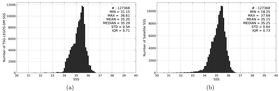
Figure 2: Histograms of SSS from TSG-LEGOS-DM (a) and SMAP-L3-RSS-V2-8DAY-RUNNING-70KM (b) considering all match-up pairs per bins of 0.1 over the South Pacific Ocean Pi-MEP region and for the full satellite product period.
