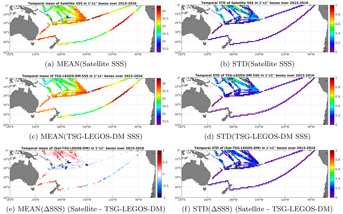
Figure 6: Temporal mean (left) and STD (right) of SSS from SMAP-L3-RSS-V2-8DAY-RUNNING-70KM (top), TSG-LEGOS-DM (middle), and of \Delta SSS (Satellite - TSG-LEGOS-DM). Only match-up pairs are used to generate these maps.
