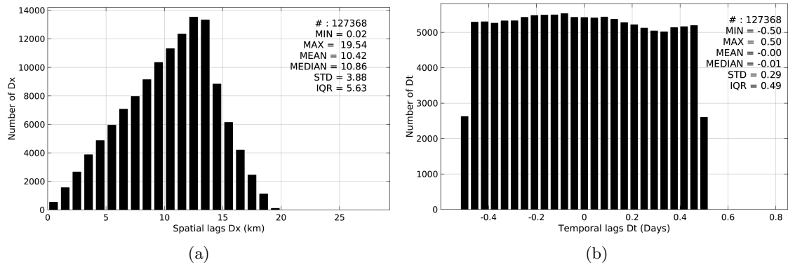
Figure 5: Histograms of the spatial (a) and temporal (b) lags between the time of the TSG-LEGOS-DM measurements and the date of the corresponding SMAP-L3-RSS-V2-8DAY-RUNNING-70KM SSS product.
