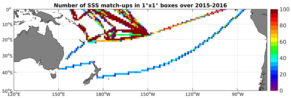
Figure 4: Number of SSS match-ups between TSG-LEGOS-DM SSS and the SMAP-L3-RSS-V2-8DAY-RUNNING-70KM SSS product for the South Pacific Ocean Pi-MEP region over 1^\circ \times 1^\circ boxes and for the full satellite product period.
