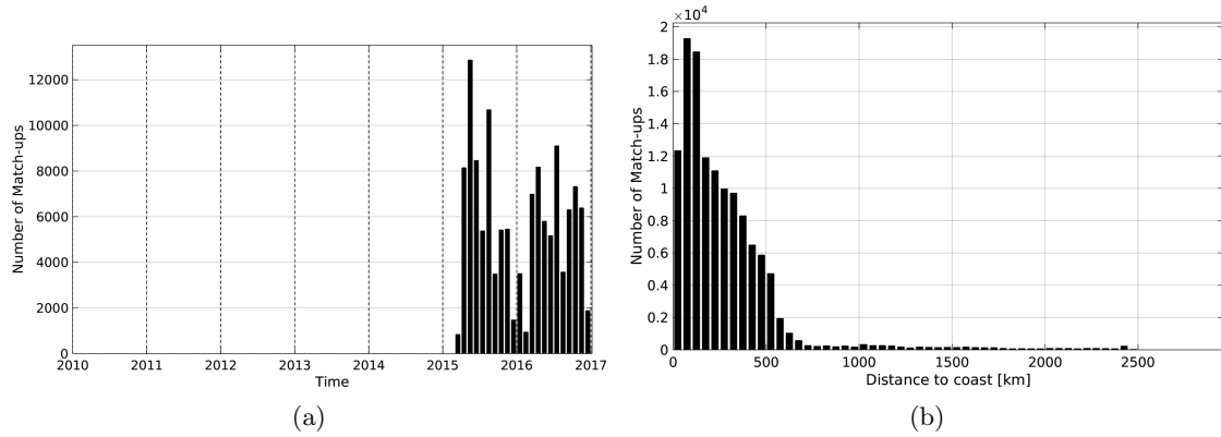
Figure 1: Number of match-ups between TSG-LEGOS-DM and SMAP-L3-RSS-V2-8DAY-RUNNING-70KM SSS as a function of time (a) and as function of the distance to coast (b) over the South Pacific Ocean Pi-MEP region and for the full satellite product period.
