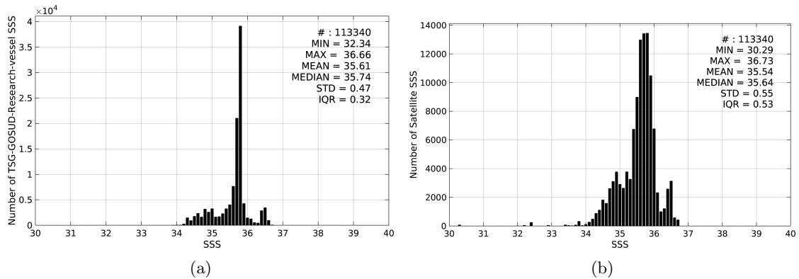
Figure 2: Histograms of SSS from TSG-GOSUD-Research-vessel (a) and SMAP-L3-RSS-V2-8DAY-RUNNING-70KM (b) considering all match-up pairs per bins of 0.1 over the South Pacific Ocean Pi-MEP region and for the full satellite product period.
