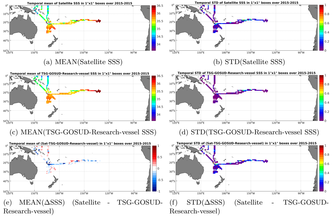
Figure 6: Temporal mean (left) and STD (right) of SSS from SMAP-L3-RSS-V2-8DAY-RUNNING-70KM (top), TSG-GOSUD-Research-vessel (middle), and of \Delta SSS (Satellite - TSG-GOSUD-Research-vessel). Only match-up pairs are used to generate these maps.
