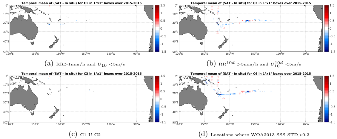
Figure 12: Temporal mean gridded over spatial boxes of size 1^\circ \times 1^\circ of \Delta SSS (SMAP-L3-RSS-V2-8DAY-RUNNING-70KM - TSG-GOSUD-Research-vessel) for 4 different subdatasets corresponding to: RR > 1\text{mm/h} and U_{10} < 5\text{m/s} (a), RR^{10d} > 5\text{mm/h} and U_{10}^{10d} < 5\text{m/s} (b), C1 U C2 (c), Locations where WOA2013 SSS STD > 0.2 (d).
