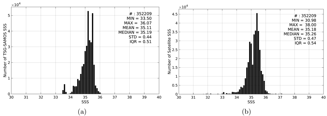
Figure 2: Histograms of SSS from TSG-SAMOS (a) and SMAP-L3-RSS-V2-MONTHLY-0.25DEG-40KM (b) considering all match-up pairs per bins of 0.1 over the South Pacific Ocean Pi-MEP region and for the full satellite product period.
