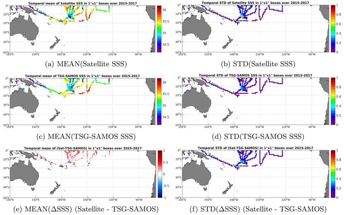
Figure 6: Temporal mean (left) and STD (right) of SSS from SMAP-L3-RSS-V2-MONTHLY-0.25DEG-40KM (top), TSG-SAMOS (middle), and of \Delta SSS (Satellite - TSG-SAMOS). Only match-up pairs are used to generate these maps.
