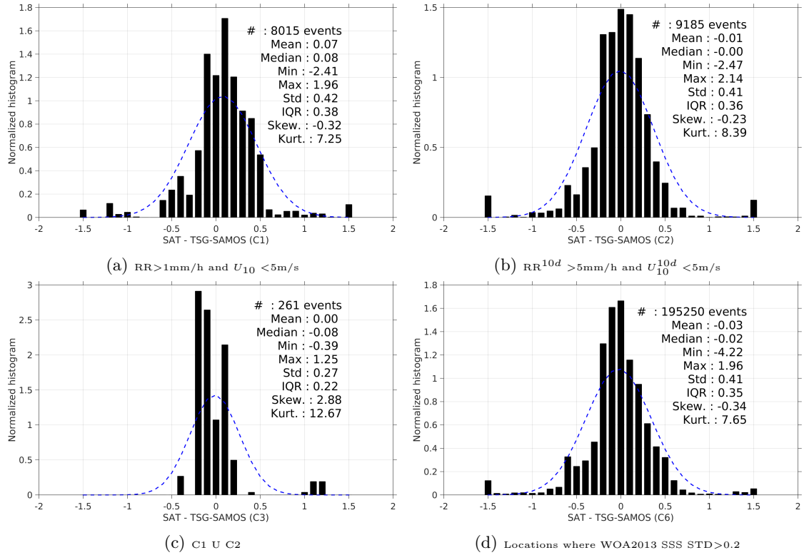
Figure 13: Normalized histogram of \Delta SSS (SMAP-L3-RSS-V2-MONTHLY-0.25DEG-40KM - TSG-SAMOS) for 6 different subdatasets corresponding to: RR > 1\text{mm/h} and U_{10} < 5\text{m/s} (a), RR^{10d} > 5\text{mm/h} and U_{10}^{10d} < 5\text{m/s} (b), C1 U C2 (c), Locations where WOA2013 SSS STD > 0.2 (d).
