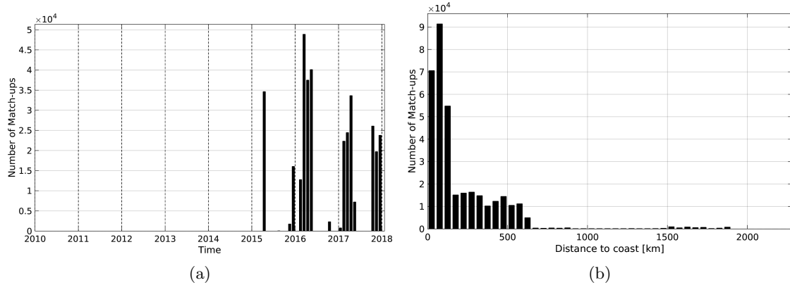
Figure 1: Number of match-ups between TSG-SAMOS and SMAP-L3-RSS-V2-MONTHLY-0.25DEG-40KM SSS as a function of time (a) and as function of the distance to coast (b) over the South Pacific Ocean Pi-MEP region and for the full satellite product period.
