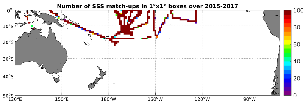
Figure 4: Number of SSS match-ups between TSG-SAMOS SSS and the SMAP-L3-RSS-V2-MONTHLY-0.25DEG-40KM SSS product for the South Pacific Ocean Pi-MEP region over 1^\circ \times 1^\circ boxes and for the full satellite product period.
