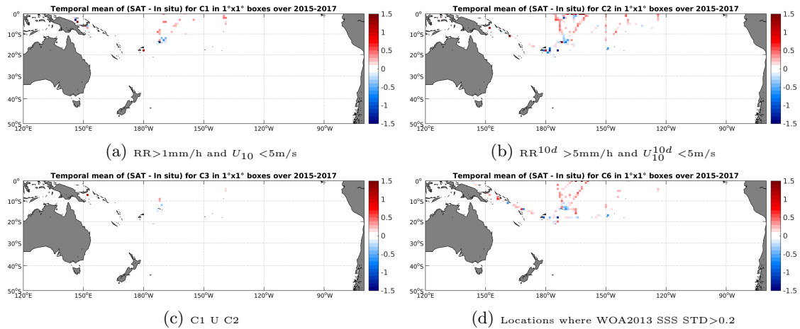
Figure 12: Temporal mean gridded over spatial boxes of size 1^\circ \times 1^\circ of \Delta SSS (SMAP-L3-RSS-V2-MONTHLY-0.25DEG-40KM - TSG-SAMOS) for 4 different subdatasets corresponding to: RR > 1\text{mm/h} and U_{10} < 5\text{m/s} (a), RR^{10d} > 5\text{mm/h} and U_{10}^{10d} < 5\text{m/s} (b), C1 U C2 (c), Locations where WOA2013 SSS STD > 0.2 (d).
