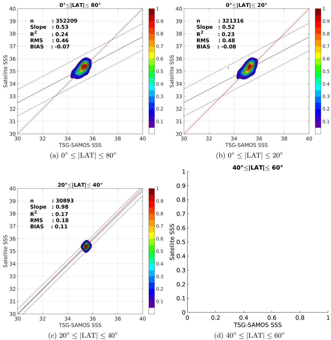
Figure 9: Contour maps of the concentration of SMAP-L3-RSS-V2-MONTHLY-0.25DEG-40KM SSS (y-axis) versus TSG-SAMOS SSS (x-axis) at match-up pairs for different latitude bands. For each plot, the red line shows x=y . The black thin and dashed lines indicate a linear fit through the data cloud and the \pm 95\% confidence levels, respectively. The number match-up pairs n , the slope and R^2 coefficient of the linear fit, the root mean square (RMS) and the mean bias between satellite and in situ data are indicated for each latitude band in each plots.
