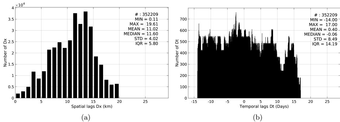
Figure 5: Histograms of the spatial (a) and temporal (b) lags between the time of the TSG-SAMOS measurements and the date of the corresponding SMAP-L3-RSS-V2-MONTHLY-0.25DEG-40KM SSS product.
