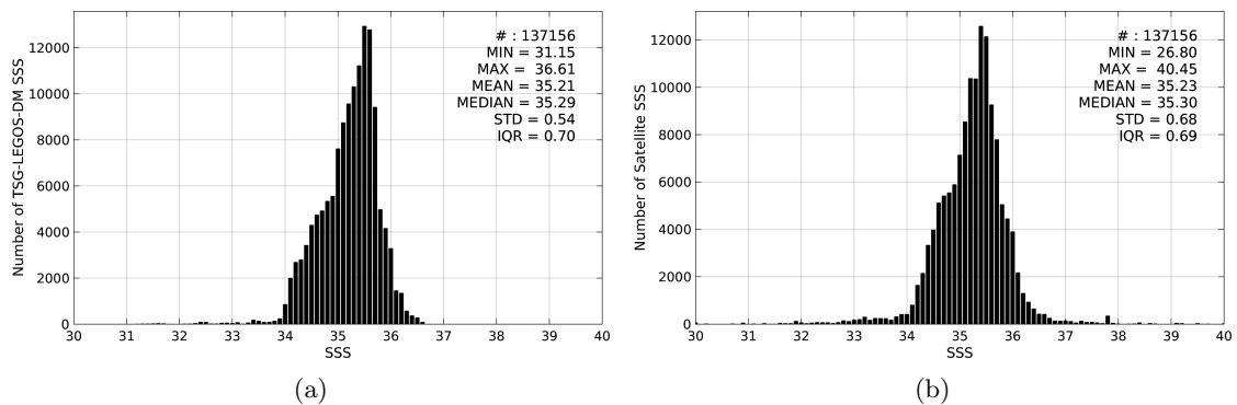
Figure 2: Histograms of SSS from TSG-LEGOS-DM (a) and SMAP-L3-RSS-V2-MONTHLY-0.25DEG-40KM (b) considering all match-up pairs per bins of 0.1 over the South Pacific Ocean Pi-MEP region and for the full satellite product period.
