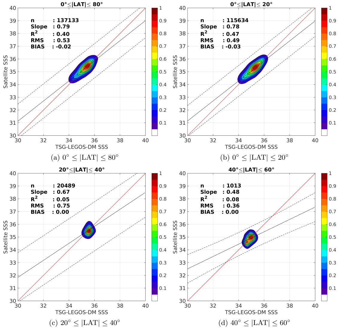
Figure 9: Contour maps of the concentration of SMAP-L3-RSS-V2-MONTHLY-0.25DEG-40KM SSS (y-axis) versus TSG-LEGOS-DM SSS (x-axis) at match-up pairs for different latitude bands. For each plot, the red line shows x=y . The black thin and dashed lines indicate a linear fit through the data cloud and the \pm 95\% confidence levels, respectively. The number match-up pairs n , the slope and R^2 coefficient of the linear fit, the root mean square (RMS) and the mean bias between satellite and in situ data are indicated for each latitude band in each plots.
