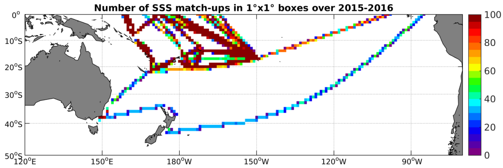
Figure 4: Number of SSS match-ups between TSG-LEGOS-DM SSS and the SMAP-L3-RSS-V2-MONTHLY-0.25DEG-40KM SSS product for the South Pacific Ocean Pi-MEP region over 1^\circ \times 1^\circ boxes and for the full satellite product period.
