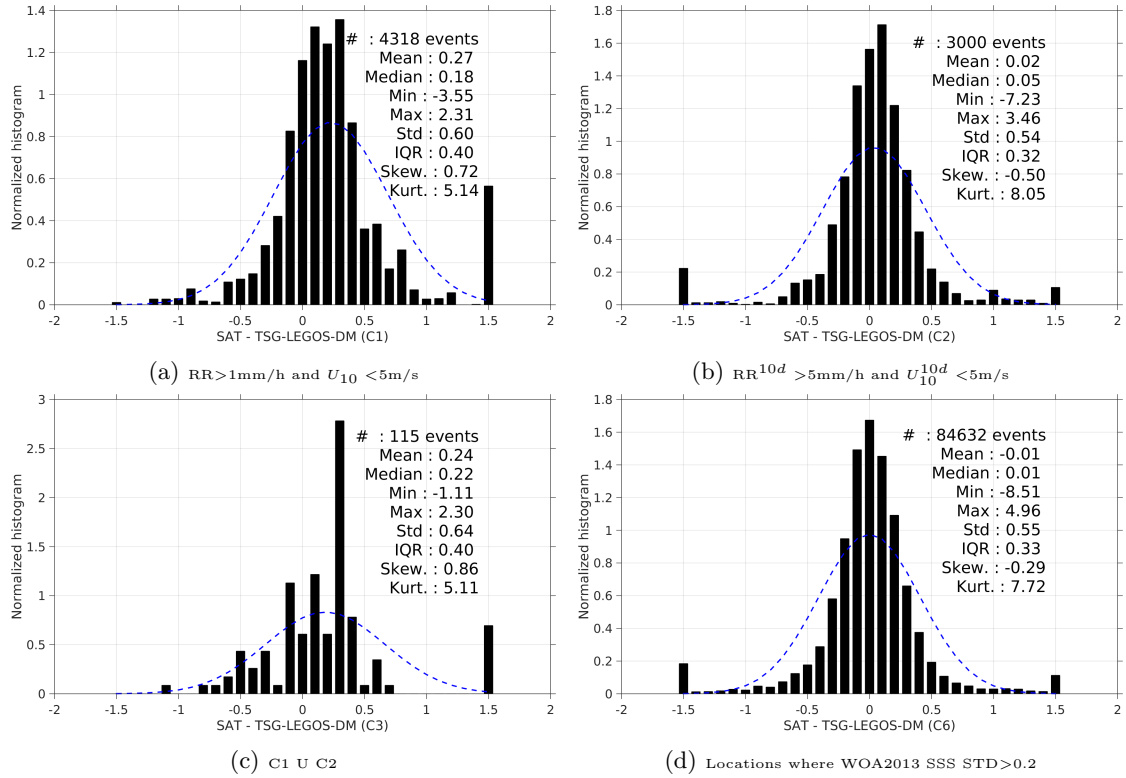
Figure 13: Normalized histogram of \Delta\text{SSS} (SMAP-L3-RSS-V2-MONTHLY-0.25DEG-40KM - TSG-LEGOS-DM) for 6 different subdatasets corresponding to: RR > 1\text{mm/h} and U_{10} < 5\text{m/s} (a), RR^{10d} > 5\text{mm/h} and U_{10}^{10d} < 5\text{m/s} (b), C1 U C2 (c), Locations where WOA2013 SSS STD > 0.2 (d).
