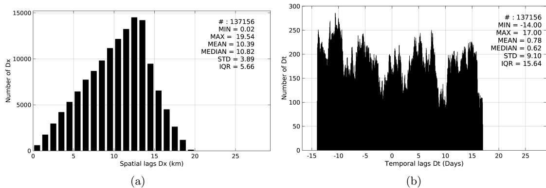
Figure 5: Histograms of the spatial (a) and temporal (b) lags between the time of the TSG-LEGOS-DM measurements and the date of the corresponding SMAP-L3-RSS-V2-MONTHLY-0.25DEG-40KM SSS product.
