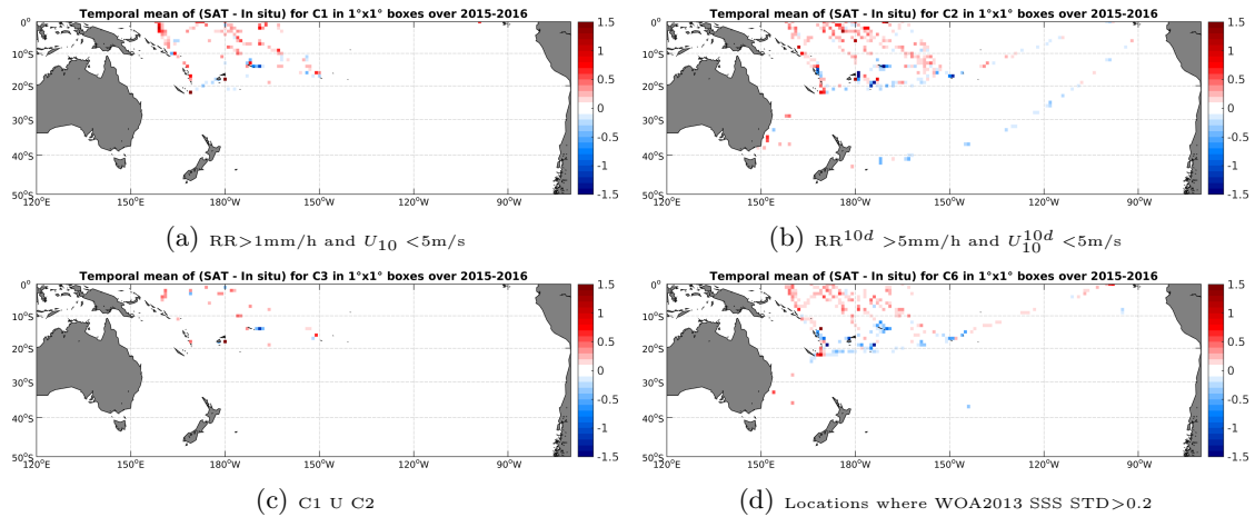
Figure 12: Temporal mean gridded over spatial boxes of size 1^\circ \times 1^\circ of \Delta SSS (SMAP-L3-RSS-V2-MONTHLY-0.25DEG-40KM - TSG-LEGOS-DM) for 4 different subdatasets corresponding to: RR > 1mm/h and U_{10} < 5\text{m/s} (a), RR^{10d} > 5\text{mm/h} and U_{10}^{10d} < 5\text{m/s} (b), C1 U C2 (c), Locations where WOA2013 SSS STD > 0.2 (d).
