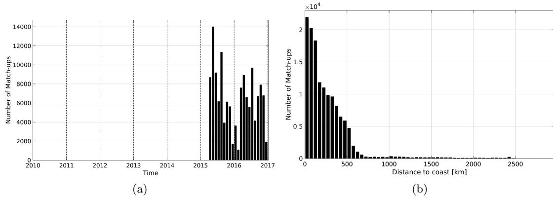
Figure 1: Number of match-ups between TSG-LEGOS-DM and SMAP-L3-RSS-V2-MONTHLY-0.25DEG-40KM SSS as a function of time (a) and as function of the distance to coast (b) over the South Pacific Ocean Pi-MEP region and for the full satellite product period.
