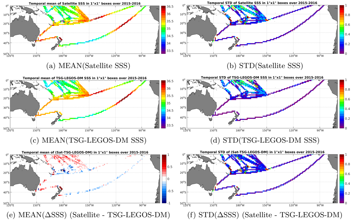
Figure 6: Temporal mean (left) and STD (right) of SSS from SMAP-L3-RSS-V2-MONTHLY-0.25DEG-40KM (top), TSG-LEGOS-DM (middle), and of \Delta SSS (Satellite - TSG-LEGOS-DM). Only match-up pairs are used to generate these maps.
