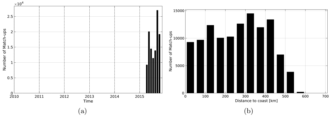
Figure 1: Number of match-ups between TSG-GOSUD-Research-vessel and SMAP-L3-RSS-V2-MONTHLY-0.25DEG-40KM SSS as a function of time (a) and as function of the distance to coast (b) over the South Pacific Ocean Pi-MEP region and for the full satellite product period.
