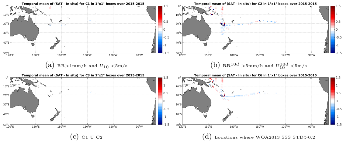
Figure 12: Temporal mean gridded over spatial boxes of size 1^\circ \times 1^\circ of \Delta SSS (SMAP-L3-RSS-V2-MONTHLY-0.25DEG-40KM - TSG-GOSUD-Research-vessel) for 4 different subdatasets corresponding to: RR > 1\text{mm/h} and U_{10} < 5\text{m/s} (a), RR^{10d} > 5\text{mm/h} and U_{10}^{10d} < 5\text{m/s} (b), C1 U C2 (c), Locations where WOA2013 SSS STD > 0.2 (d).
