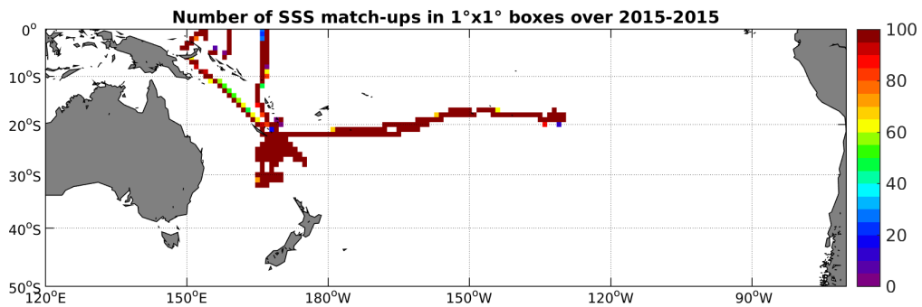
Figure 4: Number of SSS match-ups between TSG-GOSUD-Research-vessel SSS and the SMAP-L3-RSS-V2-MONTHLY-0.25DEG-40KM SSS product for the South Pacific Ocean Pi-MEP region over 1^\circ \times 1^\circ boxes and for the full satellite product period.
