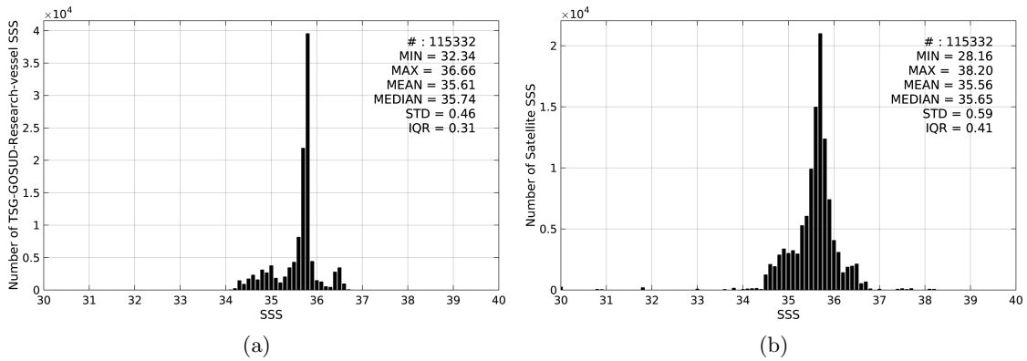
Figure 2: Histograms of SSS from TSG-GOSUD-Research-vessel (a) and SMAP-L3-RSS-V2-MONTHLY-0.25DEG-40KM (b) considering all match-up pairs per bins of 0.1 over the South Pacific Ocean Pi-MEP region and for the full satellite product period.
