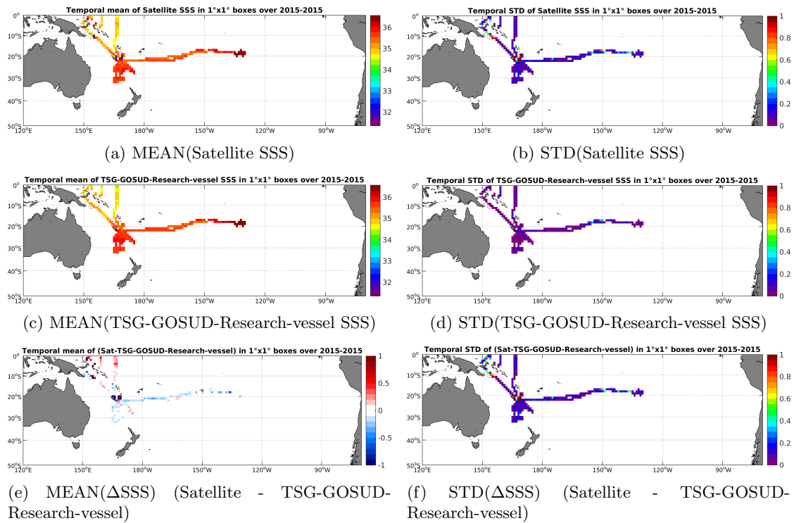
Figure 6: Temporal mean (left) and STD (right) of SSS from SMAP-L3-RSS-V2-MONTHLY-0.25DEG-40KM (top), TSG-GOSUD-Research-vessel (middle), and of \Delta SSS (Satellite - TSG-GOSUD-Research-vessel). Only match-up pairs are used to generate these maps.
