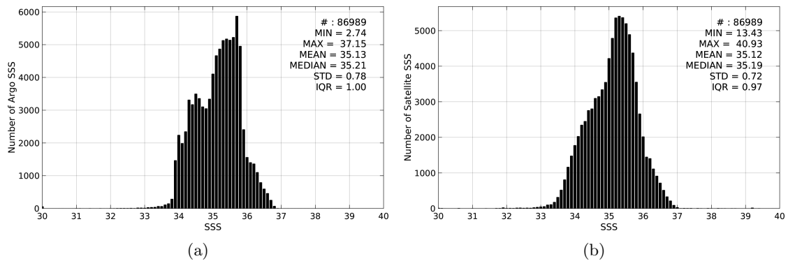
Figure 2: Histograms of SSS from Argo (a) and SMAP-L3-RSS-V2-MONTHLY-0.25DEG-40KM (b) considering all match-up pairs per bins of 0.1 over the South Pacific Ocean Pi-MEP region and for the full satellite product period.
