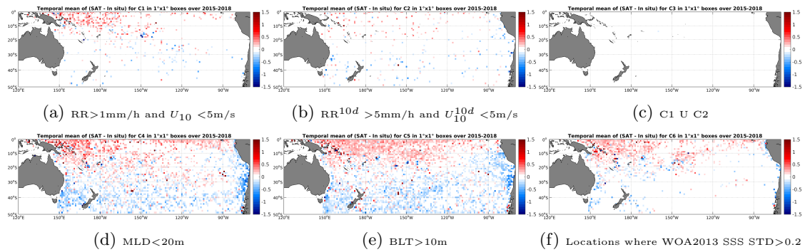
Figure 12: Temporal mean gridded over spatial boxes of size 1^\circ \times 1^\circ of \Delta SSS (SMAP-L3-RSS-V2-MONTHLY-0.25DEG-40KM - Argo) for 6 different subdatasets corresponding to:RR >1 mm/h and U_{10} < 5 m/s (a), RR ^{10d} > 5 mm/h and U_{10}^{10d} < 5 m/s (b), C1 U C2 (c),MLD <20 m (d),BLT >10 m (e),Locations where WOA2013 SSS STD >0.2 (f).
