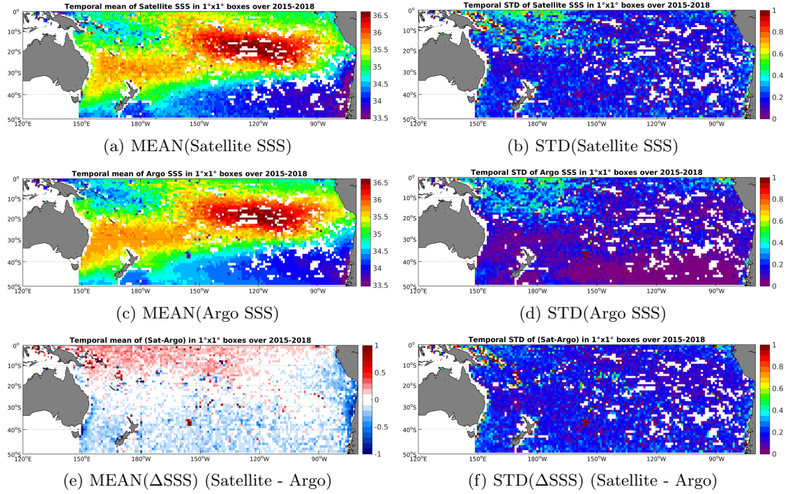
Figure 6: Temporal mean (left) and STD (right) of SSS from SMAP-L3-RSS-V2-MONTHLY-0.25DEG-40KM (top), Argo (middle), and of \Delta SSS (Satellite - Argo). Only match-up pairs are used to generate these maps.
