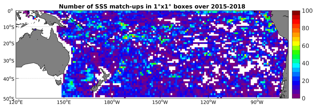
Figure 4: Number of SSS match-ups between Argo SSS and the SMAP-L3-RSS-V2-MONTHLY-0.25DEG-40KM SSS product for the South Pacific Ocean Pi-MEP region over 1^\circ \times 1^\circ boxes and for the full satellite product period.
