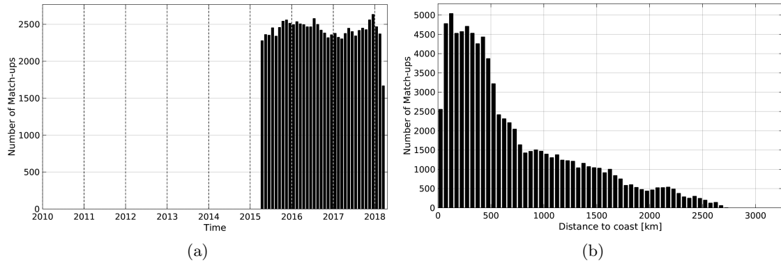
Figure 1: Number of match-ups between Argo and SMAP-L3-RSS-V2-MONTHLY-0.25DEG-40KM SSS as a function of time (a) and as function of the distance to coast (b) over the South Pacific Ocean Pi-MEP region and for the full satellite product period.
