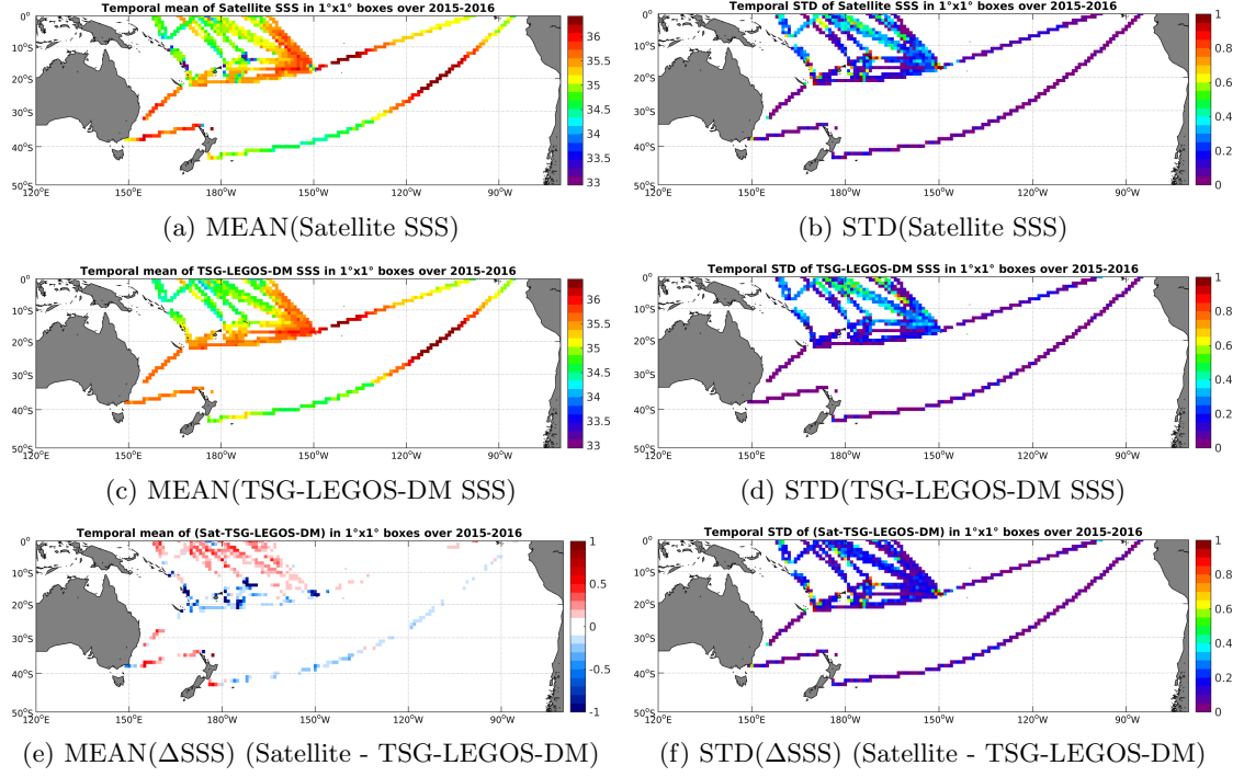
Figure 6: Temporal mean (left) and STD (right) of SSS from SMAP-L3-RSS-V2-MONTHLY-70KM (top), TSG-LEGOS-DM (middle), and of \Delta SSS (Satellite - TSG-LEGOS-DM). Only match-up pairs are used to generate these maps.
