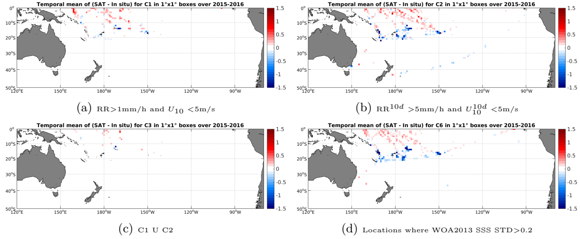
Figure 12: Temporal mean gridded over spatial boxes of size 1^\circ \times 1^\circ of \Delta SSS (SMAP-L3-RSS-V2-MONTHLY-70KM - TSG-LEGOS-DM) for 4 different subdatasets corresponding to: RR > 1 mm/h and U_{10} < 5 m/s (a), RR^{10d} > 5 mm/h and U_{10}^{10d} < 5 m/s (b), C1 U C2 (c), Locations where WOA2013 SSS STD > 0.2 (d).
