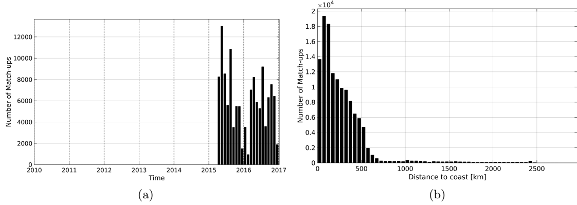
Figure 1: Number of match-ups between TSG-LEGOS-DM and SMAP-L3-RSS-V2-MONTHLY-70KM SSS as a function of time (a) and as function of the distance to coast (b) over the South Pacific Ocean Pi-MEP region and for the full satellite product period.
