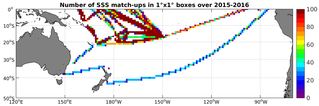
Figure 4: Number of SSS match-ups between TSG-LEGOS-DM SSS and the SMAP-L3-RSS-V2-MONTHLY-70KM SSS product for the South Pacific Ocean Pi-MEP region over 1^\circ \times 1^\circ boxes and for the full satellite product period.
