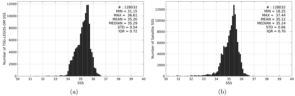
Figure 2: Histograms of SSS from TSG-LEGOS-DM (a) and SMAP-L3-RSS-V2-MONTHLY-70KM (b) considering all match-up pairs per bins of 0.1 over the South Pacific Ocean Pi-MEP region and for the full satellite product period.
