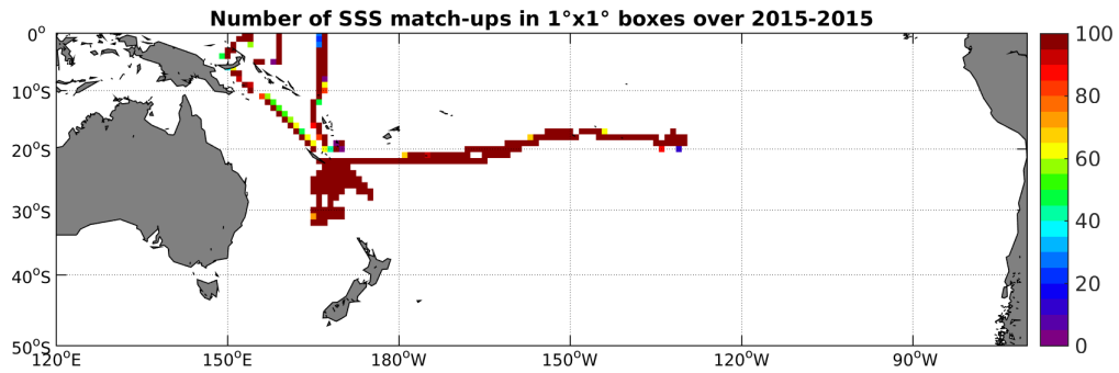
Figure 4: Number of SSS match-ups between TSG-GOSUD-Research-vessel SSS and the SMAP-L3-RSS-V2-MONTHLY-70KM SSS product for the South Pacific Ocean Pi-MEP region over 1^\circ \times 1^\circ boxes and for the full satellite product period.
