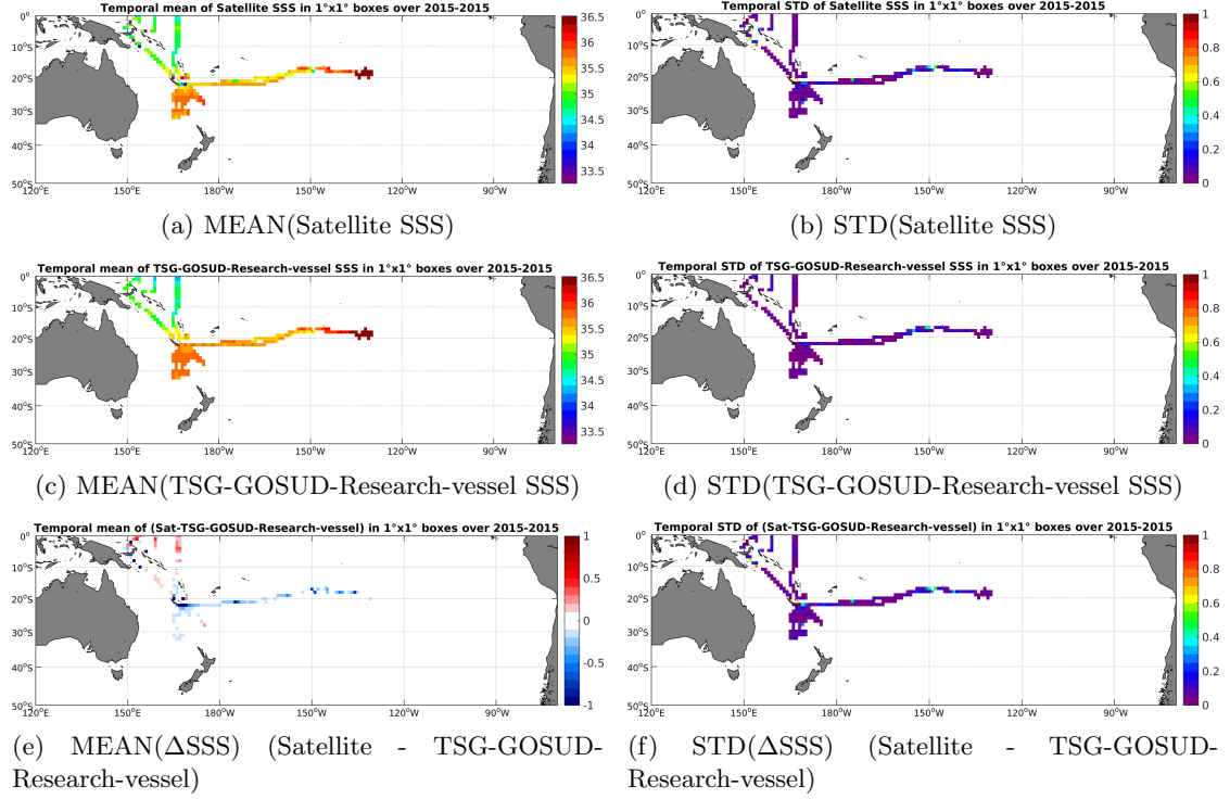
Figure 6: Temporal mean (left) and STD (right) of SSS from SMAP-L3-RSS-V2-MONTHLY-70KM (top), TSG-GOSUD-Research-vessel (middle), and of \Delta SSS (Satellite - TSG-GOSUD-Research-vessel). Only match-up pairs are used to generate these maps.
