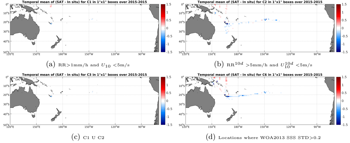
Figure 12: Temporal mean gridded over spatial boxes of size 1^\circ \times 1^\circ of \Delta SSS (SMAP-L3-RSS-V2-MONTHLY-70KM - TSG-GOSUD-Research-vessel) for 4 different subdatasets corresponding to: RR > 1mm/h and U_{10} < 5 m/s (a), RR^{10d} > 5 mm/h and U_{10}^{10d} < 5 m/s (b), C1 U C2 (c), Locations where WOA2013 SSS STD > 0.2 (d).
