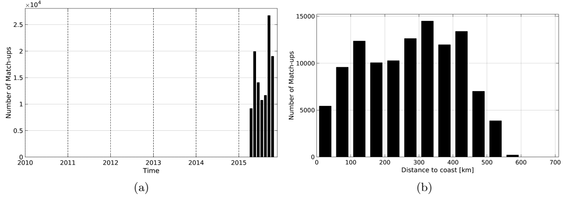
Figure 1: Number of match-ups between TSG-GOSUD-Research-vessel and SMAP-L3-RSS-V2-MONTHLY-70KM SSS as a function of time (a) and as function of the distance to coast (b) over the South Pacific Ocean Pi-MEP region and for the full satellite product period.
