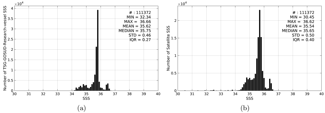
Figure 2: Histograms of SSS from TSG-GOSUD-Research-vessel (a) and SMAP-L3-RSS-V2-MONTHLY-70KM (b) considering all match-up pairs per bins of 0.1 over the South Pacific Ocean Pi-MEP region and for the full satellite product period.
