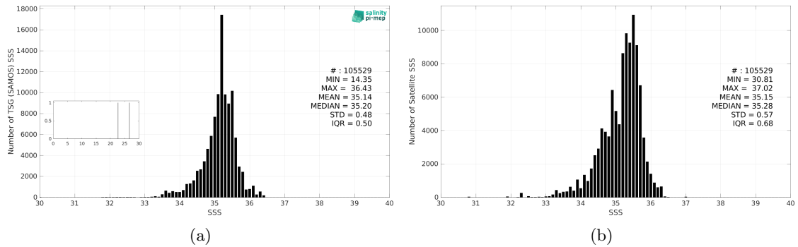
Figure 3: Histograms of SSS from TSG (SAMOS) (a) and SMAP SSS L3 v5.0 - 8-Day running (JPL) (b) considering all match-up pairs per bins of 0.1 over the South Pacific Ocean Pi-MEP region and for the full satellite product period.
