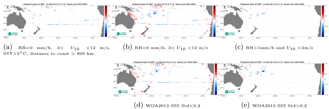
Figure 14: Temporal mean gridded over spatial boxes of size 1^\circ \times 1^\circ of \Delta SSS (SMAP SSS L3 v5.0 - 8-Day running (JPL) - TSG (SAMOS)) for 5 different subdatasets corresponding to:RR=0 mm/h, 3 < U_{10} < 12 m/s, SST >5^\circ\text{C} , distance to coast > 800 km (a), RR=0 mm/h, 3 < U_{10} < 12 m/s (b), RR >1 mm/h and U_{10} < 4 m/s (c), WOA2013 SSS Std <0.2 (d), WOA2013 SSS Std >0.2 (e).
