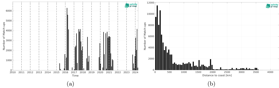
Figure 2: Number of match-ups between TSG (SAMOS) and SMAP SSS L3 v5.0 - 8-Day running (JPL) SSS as a function of time (a) and as function of the distance to coast (b) over the South Pacific Ocean Pi-MEP region and for the full satellite product period.
