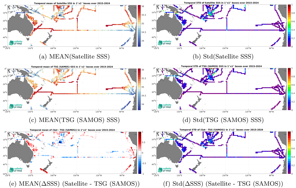
Figure 7: Temporal mean (left) and Std (right) of SSS from SMAP SSS L3 v5.0 - 8-Day running (JPL) (top), TSG (SAMOS) (middle), and of \Delta SSS (Satellite - TSG (SAMOS)). Only match-up pairs are used to generate these maps.
