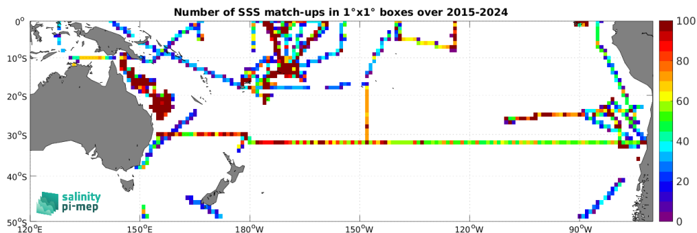
Figure 5: Number of SSS match-ups between TSG (SAMOS) SSS and the SMAP SSS L3 v5.0 - 8-Day running (JPL) SSS product for the South Pacific Ocean Pi-MEP region over 1^\circ \times 1^\circ boxes and for the full satellite product period.
