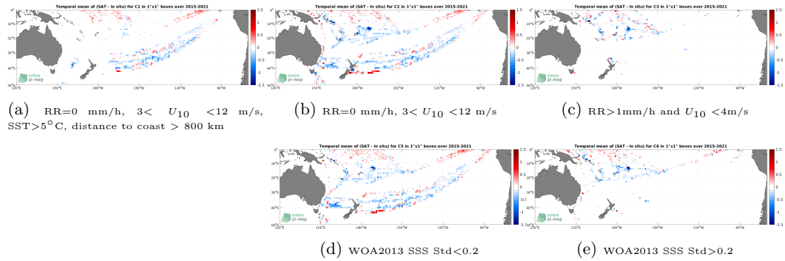
Figure 12: Temporal mean gridded over spatial boxes of size 1^\circ \times 1^\circ of \Delta SSS (SMAP SSS L3 v5.0 - 8-Day running (JPL) - TSG (LEGOS-DM)) for 5 different subdatasets corresponding to:RR=0 mm/h, 3 < U_{10} < 12 m/s, SST >5^\circ\text{C} , distance to coast > 800 km (a), RR=0 mm/h, 3 < U_{10} < 12 m/s (b), RR >1 mm/h and U_{10} < 4 m/s (c), WOA2013 SSS Std <0.2 (d), WOA2013 SSS Std >0.2 (e).
