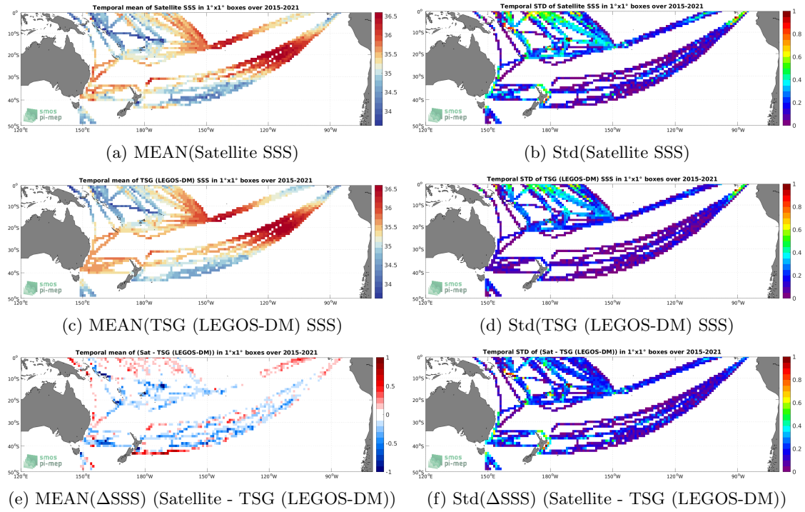
Figure 6: Temporal mean (left) and Std (right) of SSS from SMAP SSS L3 v5.0 - 8-Day running (JPL) (top), TSG (LEGOS-DM) (middle), and of \Delta SSS (Satellite - TSG (LEGOS-DM)). Only match-up pairs are used to generate these maps.
