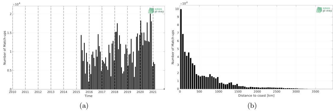
Figure 1: Number of match-ups between TSG (LEGOS-DM) and SMAP SSS L3 v5.0 - 8-Day running (JPL) SSS as a function of time (a) and as function of the distance to coast (b) over the South Pacific Ocean Pi-MEP region and for the full satellite product period.
