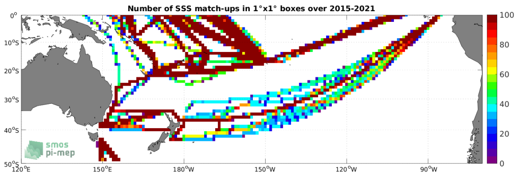
Figure 4: Number of SSS match-ups between TSG (LEGOS-DM) SSS and the SMAP SSS L3 v5.0 - 8-Day running (JPL) SSS product for the South Pacific Ocean Pi-MEP region over 1^\circ \times 1^\circ boxes and for the full satellite product period.
