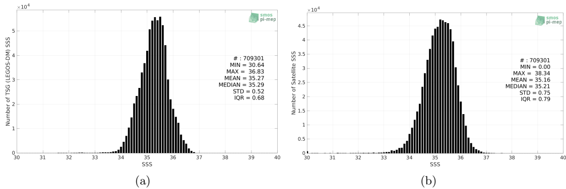
Figure 2: Histograms of SSS from TSG (LEGOS-DM) (a) and SMAP SSS L3 v5.0 - 8-Day running (JPL) (b) considering all match-up pairs per bins of 0.1 over the South Pacific Ocean Pi-MEP region and for the full satellite product period.
