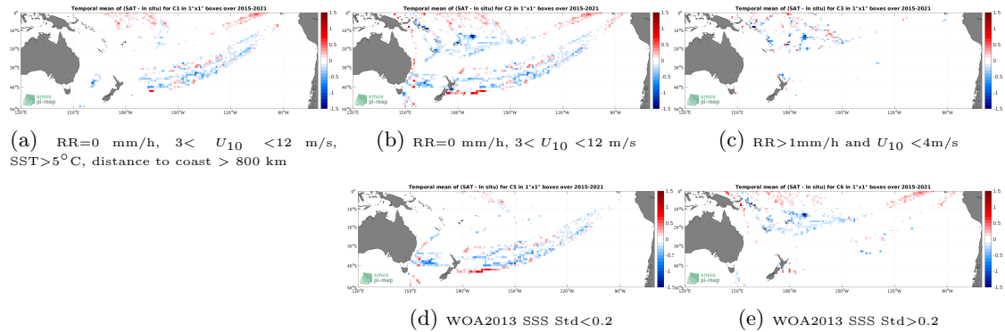
Figure 12: Temporal mean gridded over spatial boxes of size 1^\circ \times 1^\circ of \Delta\text{SSS} (SMAP SSS L3 v5.0 - 8-Day running (JPL) - TSG (LEGOS-DM)) for 5 different subdatasets corresponding to: \text{RR}=0 mm/h, 3 < U_{10} < 12 m/s, \text{SST} > 5^\circ\text{C} , distance to coast > 800 km (a), \text{RR}=0 mm/h, 3 < U_{10} < 12 m/s (b), \text{RR} > 1\text{mm/h} and U_{10} < 4\text{m/s} (c), WOA2013 SSS Std < 0.2 (d), WOA2013 SSS Std > 0.2 (e).
