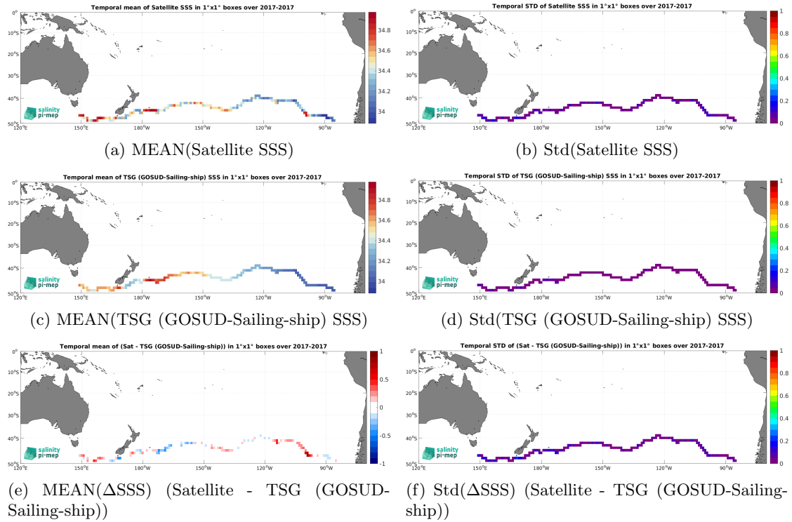
Figure 7: Temporal mean (left) and Std (right) of SSS from SMAP SSS L3 v5.0 - 8-Day running (JPL) (top), TSG (GOSUD-Sailing-ship) (middle), and of \Delta SSS (Satellite - TSG (GOSUD-Sailing-ship)). Only match-up pairs are used to generate these maps.
