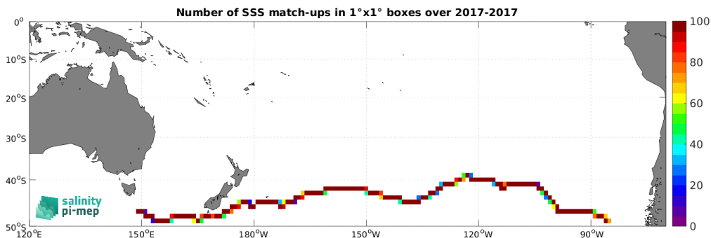
Figure 5: Number of SSS match-ups between TSG (GOSUD-Sailing-ship) SSS and the SMAP SSS L3 v5.0 - 8-Day running (JPL) SSS product for the South Pacific Ocean Pi-MEP region over 1^\circ \times 1^\circ boxes and for the full satellite product period.
