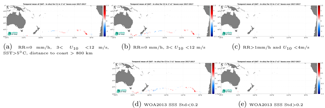
Figure 14: Temporal mean gridded over spatial boxes of size 1^\circ \times 1^\circ of \Delta\text{SSS} (SMAP SSS L3 v5.0 - 8-Day running (JPL) - TSG (GOSUD-Sailing-ship)) for 5 different subdatasets corresponding to:RR=0 mm/h, 3 < U_{10} < 12 m/s, SST>5°C, distance to coast > 800 km (a), RR=0 mm/h, 3 < U_{10} < 12 m/s (b), RR>1mm/h and U_{10} < 4 m/s (c), WOA2013 SSS Std<0.2 (d), WOA2013 SSS Std>0.2 (e).
