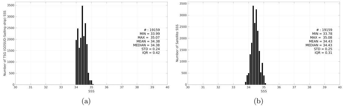
Figure 3: Histograms of SSS from TSG (GOSUD-Sailing-ship) (a) and SMAP SSS L3 v5.0 - 8-Day running (JPL) (b) considering all match-up pairs per bins of 0.1 over the South Pacific Ocean Pi-MEP region and for the full satellite product period.
