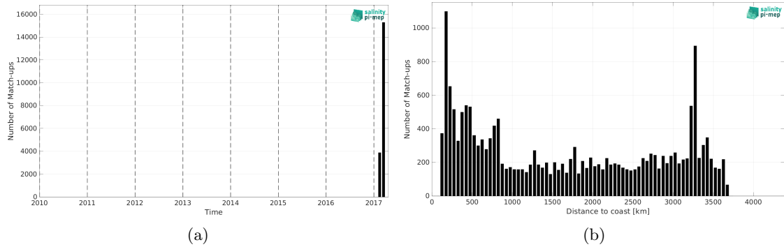
Figure 2: Number of match-ups between TSG (GOSUD-Sailing-ship) and SMAP SSS L3 v5.0 - 8-Day running (JPL) SSS as a function of time (a) and as function of the distance to coast (b) over the South Pacific Ocean Pi-MEP region and for the full satellite product period.
