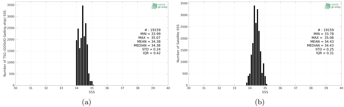
Figure 2: Histograms of SSS from TSG (GOSUD-Sailing-ship) (a) and SMAP SSS L3 v5.0 - 8-Day running (JPL) (b) considering all match-up pairs per bins of 0.1 over the South Pacific Ocean Pi-MEP region and for the full satellite product period.
