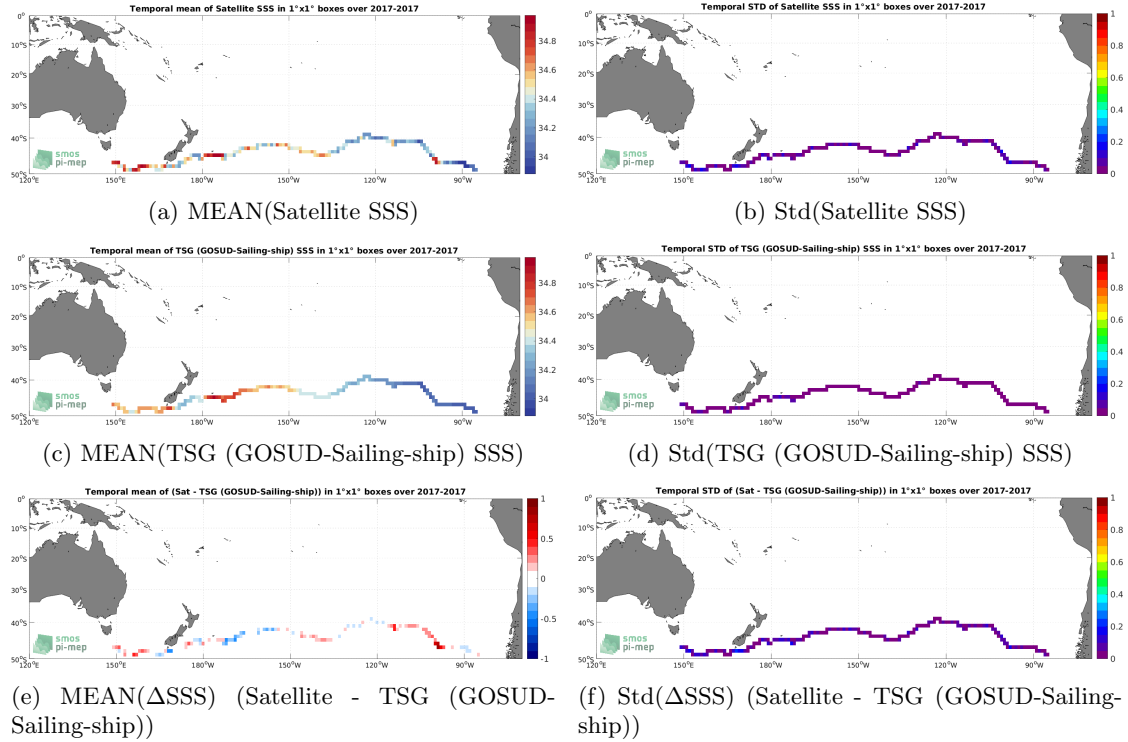
Figure 6: Temporal mean (left) and Std (right) of SSS from SMAP SSS L3 v5.0 - 8-Day running (JPL) (top), TSG (GOSUD-Sailing-ship) (middle), and of \Delta SSS (Satellite - TSG (GOSUD-Sailing-ship)). Only match-up pairs are used to generate these maps.
