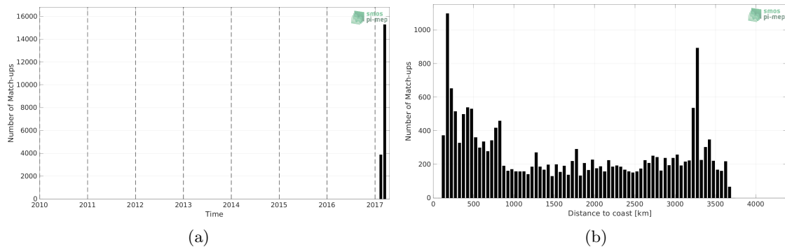
Figure 1: Number of match-ups between TSG (GOSUD-Sailing-ship) and SMAP SSS L3 v5.0 - 8-Day running (JPL) SSS as a function of time (a) and as function of the distance to coast (b) over the South Pacific Ocean Pi-MEP region and for the full satellite product period.
