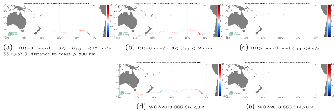
Figure 12: Temporal mean gridded over spatial boxes of size 1^\circ \times 1^\circ of \Delta SSS (SMAP SSS L3 v5.0 - 8-Day running (JPL) - TSG (GOSUD-Sailing-ship)) for 5 different subdatasets corresponding to:RR=0 mm/h, 3 < U_{10} < 12 m/s, SST >5^\circ\text{C} , distance to coast > 800 km (a), RR=0 mm/h, 3 < U_{10} < 12 m/s (b), RR >1 mm/h and U_{10} < 4 m/s (c), WOA2013 SSS Std <0.2 (d), WOA2013 SSS Std >0.2 (e).
