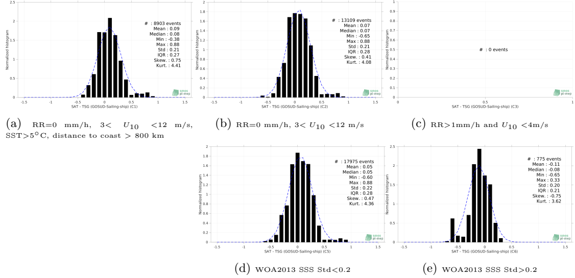
Figure 13: Normalized histogram of \Delta\text{SSS} (SMAP SSS L3 v5.0 - 8-Day running (JPL) - TSG (GOSUD-Sailing-ship)) for 5 different subdatasets corresponding to: RR=0 mm/h, 3 < U_{10} < 12 m/s, SST >5^{\circ}\text{C} , distance to coast > 800 km (a), RR=0 mm/h, 3 < U_{10} < 12 m/s (b), RR >1 mm/h and U_{10} < 4 m/s (c), WOA2013 SSS Std <0.2 (d), WOA2013 SSS Std >0.2 (e).
