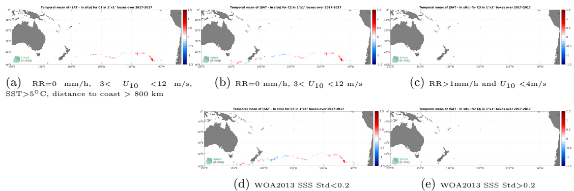
Figure 12: Temporal mean gridded over spatial boxes of size 1^\circ \times 1^\circ of \Delta\text{SSS} (SMAP SSS L3 v5.0 - 8-Day running (JPL) - TSG (GOSUD-Sailing-ship)) for 5 different subdatasets corresponding to:RR=0 mm/h, 3 < U_{10} < 12 m/s, SST>5°C, distance to coast > 800 km (a), RR=0 mm/h, 3 < U_{10} < 12 m/s (b), RR>1mm/h and U_{10} < 4 m/s (c), WOA2013 SSS Std<0.2 (d), WOA2013 SSS Std>0.2 (e).
