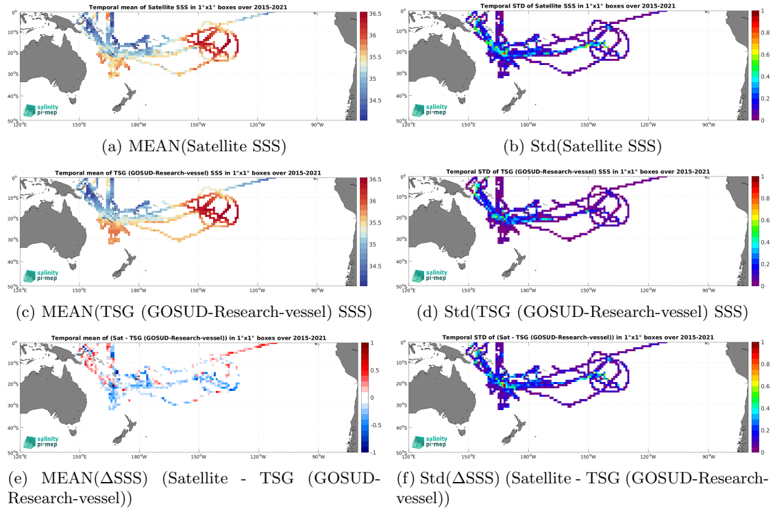
Figure 7: Temporal mean (left) and Std (right) of SSS from SMAP SSS L3 v5.0 - 8-Day running (JPL) (top), TSG (GOSUD-Research-vessel) (middle), and of \Delta SSS (Satellite - TSG (GOSUD-Research-vessel)). Only match-up pairs are used to generate these maps.
