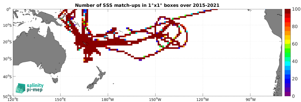
Figure 5: Number of SSS match-ups between TSG (GOSUD-Research-vessel) SSS and the SMAP SSS L3 v5.0 - 8-Day running (JPL) SSS product for the South Pacific Ocean Pi-MEP region over 1^\circ \times 1^\circ boxes and for the full satellite product period.
