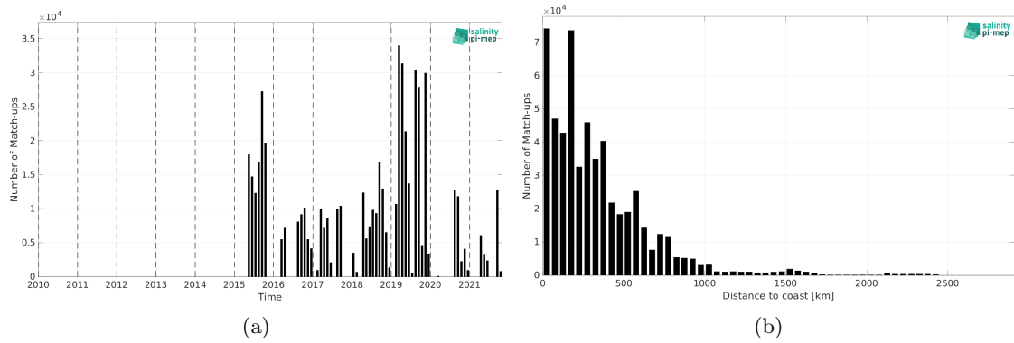
Figure 2: Number of match-ups between TSG (GOSUD-Research-vessel) and SMAP SSS L3 v5.0 - 8-Day running (JPL) SSS as a function of time (a) and as function of the distance to coast (b) over the South Pacific Ocean Pi-MEP region and for the full satellite product period.
