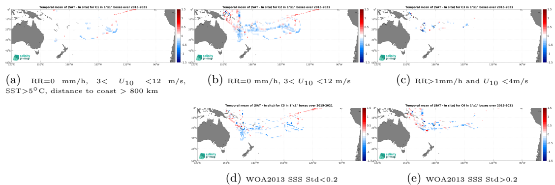
Figure 14: Temporal mean gridded over spatial boxes of size 1^\circ \times 1^\circ of \Delta\text{SSS} (SMAP SSS L3 v5.0 - 8-Day running (JPL) - TSG (GOSUD-Research-vessel)) for 5 different subdatasets corresponding to:RR=0 mm/h, 3 < U_{10} < 12 m/s, SST >5^\circ\text{C} , distance to coast > 800 km (a), RR=0 mm/h, 3 < U_{10} < 12 m/s (b), RR >1 mm/h and U_{10} < 4 m/s (c), WOA2013 SSS Std <0.2 (d), WOA2013 SSS Std >0.2 (e).
