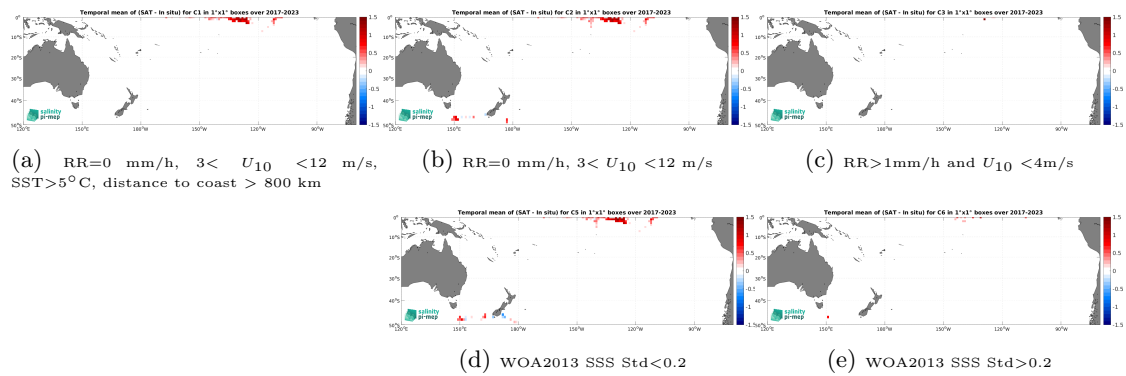
Figure 14: Temporal mean gridded over spatial boxes of size 1^\circ \times 1^\circ of \Delta\text{SSS} (SMAP SSS L3 v5.0 - 8-Day running (JPL) - Saikrone) for 5 different subdatasets corresponding to:RR=0 mm/h, 3 < U_{10} < 12 m/s, SST>5°C, distance to coast > 800 km (a), RR=0 mm/h, 3 < U_{10} < 12 m/s (b), RR>1mm/h and U_{10} < 4 m/s (c), WOA2013 SSS Std<0.2 (d), WOA2013 SSS Std>0.2 (e).
