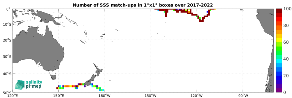
Figure 5: Number of SSS match-ups between Saildrone SSS and the SMAP SSS L3 v5.0 - 8-Day running (JPL) SSS product for the South Pacific Ocean Pi-MEP region over 1^\circ \times 1^\circ boxes and for the full satellite product period.
