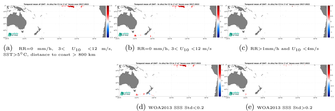
Figure 14: Temporal mean gridded over spatial boxes of size 1^\circ \times 1^\circ of \Delta SSS (SMAP SSS L3 v5.0 - 8-Day running (JPL) - Saifdrone) for 5 different subdatasets corresponding to:RR=0 mm/h, 3 < U_{10} < 12 m/s, SST >5^\circ\text{C} , distance to coast > 800 km (a), RR=0 mm/h, 3 < U_{10} < 12 m/s (b), RR >1 mm/h and U_{10} < 4 m/s (c), WOA2013 SSS Std <0.2 (d), WOA2013 SSS Std >0.2 (e).
