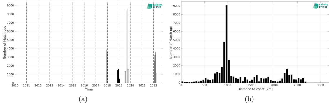
Figure 2: Number of match-ups between Saildrone and SMAP SSS L3 v5.0 - 8-Day running (JPL) SSS as a function of time (a) and as function of the distance to coast (b) over the South Pacific Ocean Pi-MEP region and for the full satellite product period.
