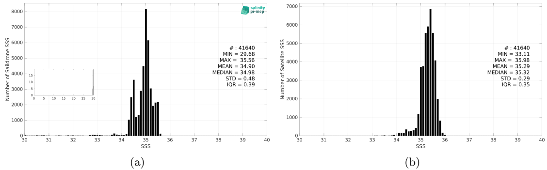
Figure 3: Histograms of SSS from Saildrone (a) and SMAP SSS L3 v5.0 - 8-Day running (JPL) (b) considering all match-up pairs per bins of 0.1 over the South Pacific Ocean Pi-MEP region and for the full satellite product period.
