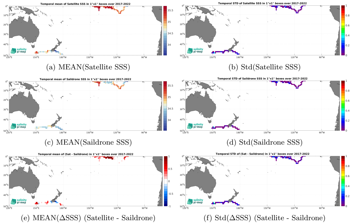
Figure 7: Temporal mean (left) and Std (right) of SSS from SMAP SSS L3 v5.0 - 8-Day running (JPL) (top), Saildrone (middle), and of \Delta SSS (Satellite - Saildrone). Only match-up pairs are used to generate these maps.
