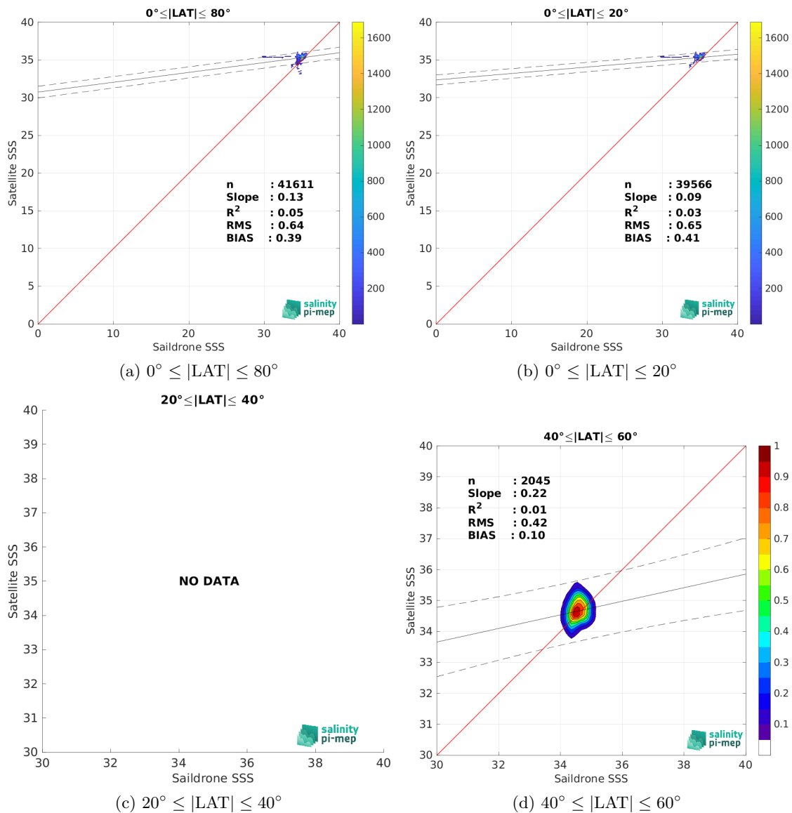
Figure 9: Contour maps of the concentration of SMAP SSS L3 v5.0 - 8-Day running (JPL) SSS (y-axis) versus Sairdrone SSS (x-axis) at match-up pairs for different latitude bands. For each plot, the red line shows x=y . The black thin and dashed lines indicate a linear fit through the data cloud and the \pm 95\% confidence levels, respectively. The number match-up pairs n , the slope and R^2 coefficient of the linear fit, the root mean square (RMS) and the mean bias between satellite and in situ data are indicated for each latitude band in each plots.
