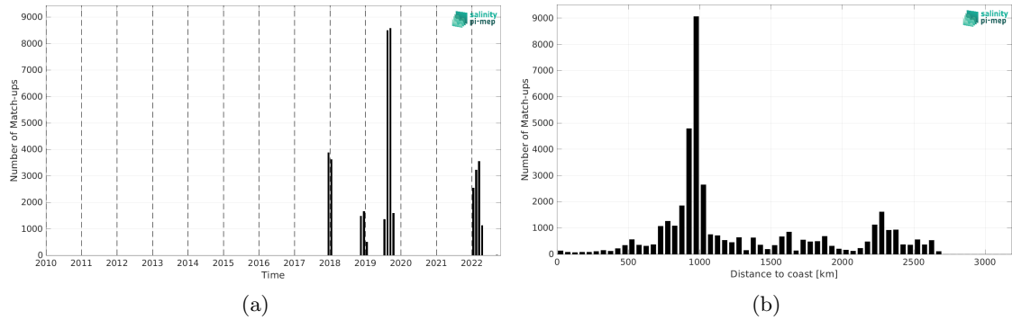
Figure 1: Number of match-ups between Sairdron and SMAP SSS L3 v5.0 - 8-Day running (JPL) SSS as a function of time (a) and as function of the distance to coast (b) over the South Pacific Ocean Pi-MEP region and for the full satellite product period.
