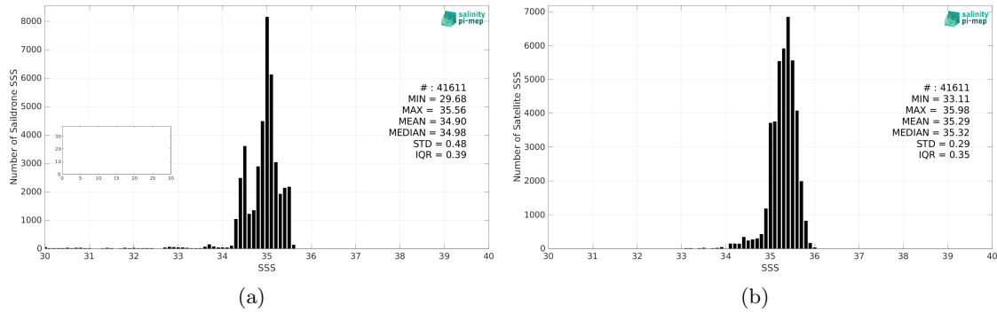
Figure 2: Histograms of SSS from Sairdron (a) and SMAP SSS L3 v5.0 - 8-Day running (JPL) (b) considering all match-up pairs per bins of 0.1 over the South Pacific Ocean Pi-MEP region and for the full satellite product period.
