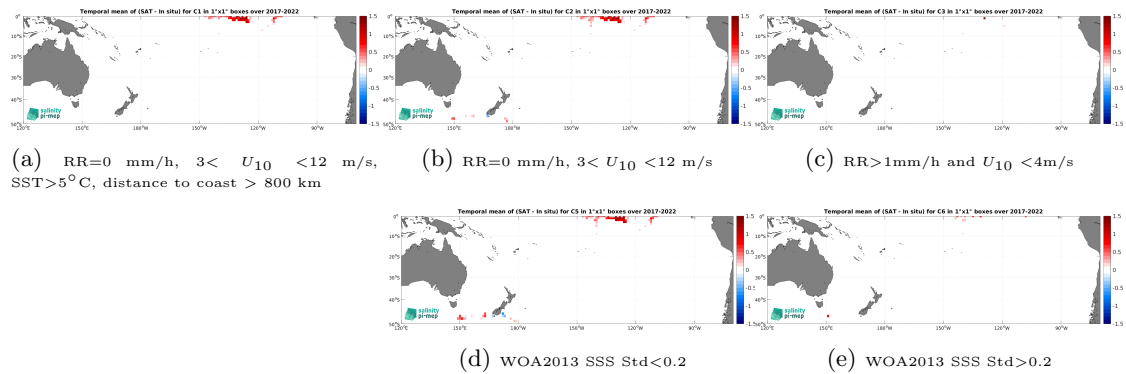
Figure 12: Temporal mean gridded over spatial boxes of size 1^\circ \times 1^\circ of \Delta SSS (SMAP SSS L3 v5.0 - 8-Day running (JPL) - Saildrone) for 5 different subdatasets corresponding to:RR=0 mm/h, 3 < U_{10} < 12 m/s, SST >5^\circ\text{C} , distance to coast > 800 km (a), RR=0 mm/h, 3 < U_{10} < 12 m/s (b), RR >1 mm/h and U_{10} < 4 m/s (c), WOA2013 SSS Std <0.2 (d), WOA2013 SSS Std >0.2 (e).
