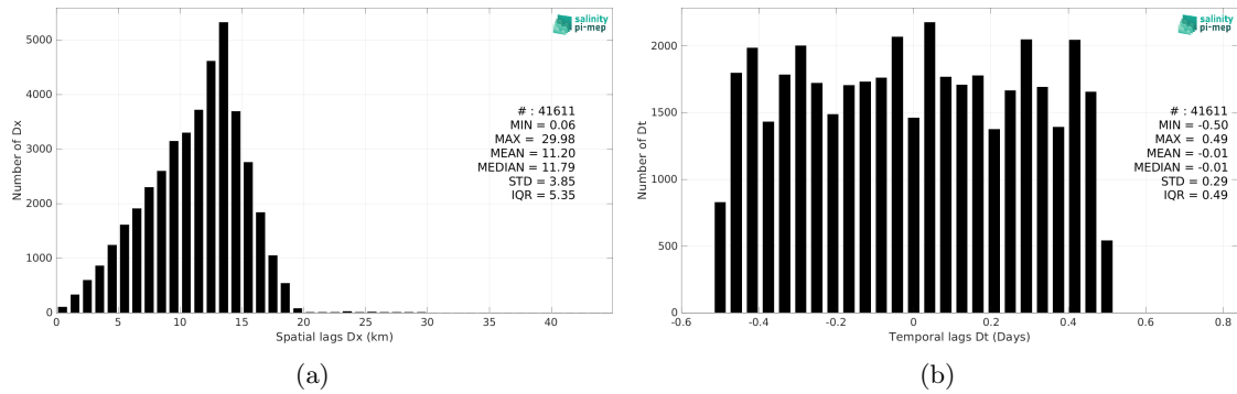
Figure 5: Histograms of the spatial (a) and temporal (b) lags between the location/time of the Sairdronc measurement and the date of the corresponding SMAP SSS L3 v5.0 - 8-Day running (JPL) SSS pixel.
