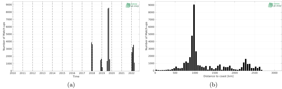
Figure 1: Number of match-ups between Saildrone and SMAP SSS L3 v5.0 - 8-Day running (JPL) SSS as a function of time (a) and as function of the distance to coast (b) over the South Pacific Ocean Pi-MEP region and for the full satellite product period.
