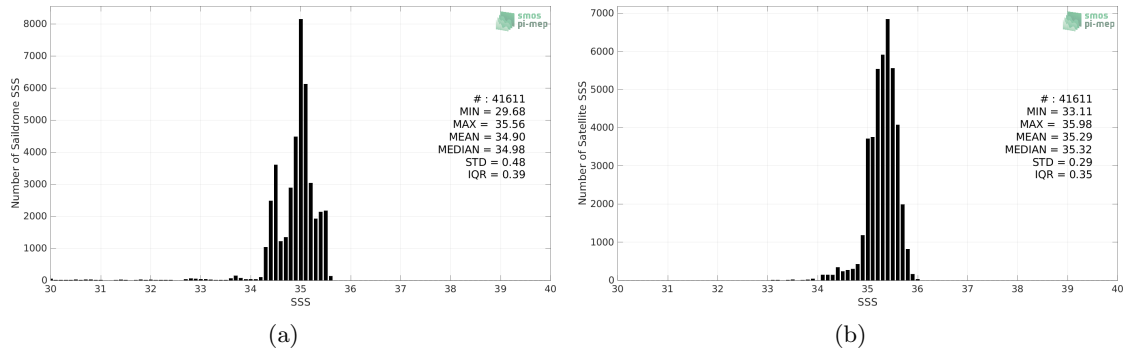
Figure 2: Histograms of SSS from Saildrone (a) and SMAP SSS L3 v5.0 - 8-Day running (JPL) (b) considering all match-up pairs per bins of 0.1 over the South Pacific Ocean Pi-MEP region and for the full satellite product period.
