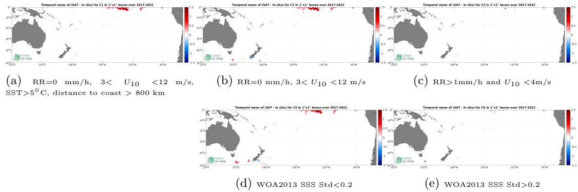
Figure 12: Temporal mean gridded over spatial boxes of size 1^\circ \times 1^\circ of \Delta SSS (SMAP SSS L3 v5.0 - 8-Day running (JPL) - Saifdrone) for 5 different subdatasets corresponding to:RR=0 mm/h, 3 < U_{10} < 12 m/s, SST >5^\circ\text{C} , distance to coast > 800 km (a), RR=0 mm/h, 3 < U_{10} < 12 m/s (b), RR >1 mm/h and U_{10} < 4 m/s (c), WOA2013 SSS Std <0.2 (d), WOA2013 SSS Std >0.2 (e).
